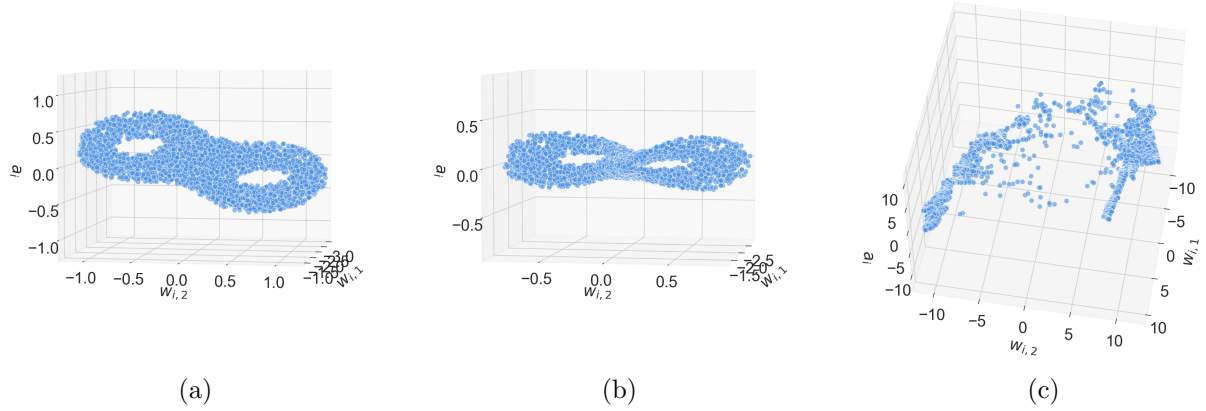
Figure 8: Topology of a 3D neural network with momentum gradient descent. The neurons are initialized on a genus-2 surface and optimized with momentum GD. The camera angle is manually adjusted to better visualize the structure of the point cloud.
