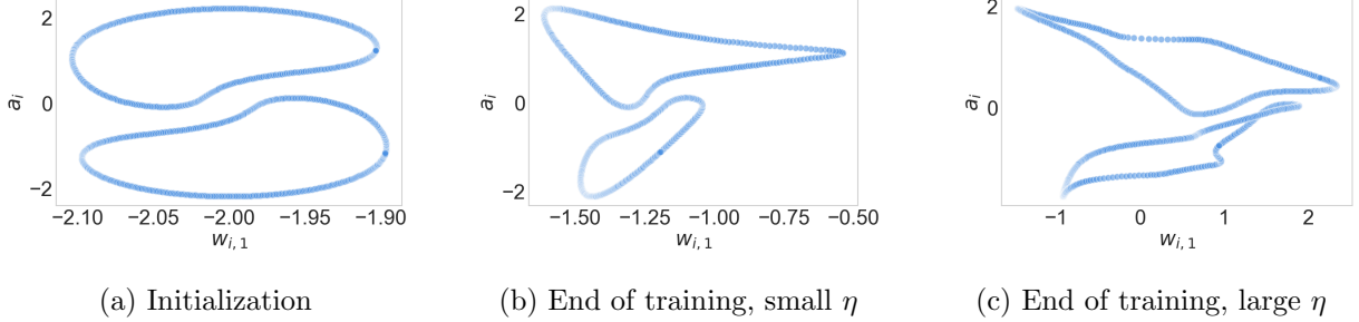
Figure 6: Topology of a 2D neural network with GD and disjoint genus-1 initialization. The neurons are initialized on the disjoint union of two genus-1 surfaces and optimized with GD.
