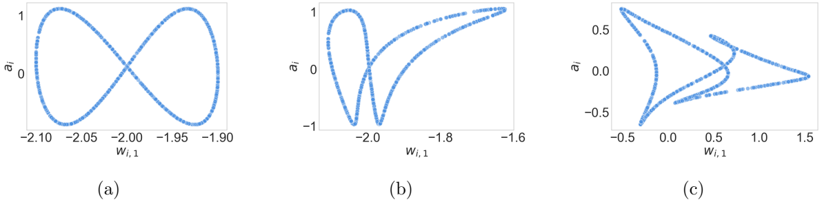
Figure 7: Topology of a 2D neural network with momentum gradient descent. The neurons are initialized on a genus-2 surface and optimized with momentum GD.
