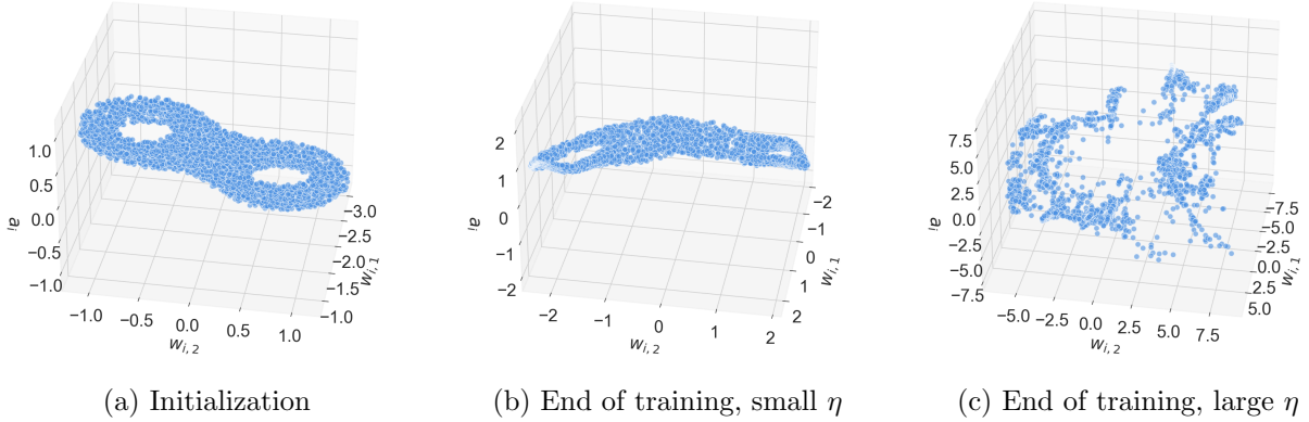
Figure 4: Topology of a 3D neural network with GD. The neurons are initialized on a genus-2 surface and optimized with GD.
