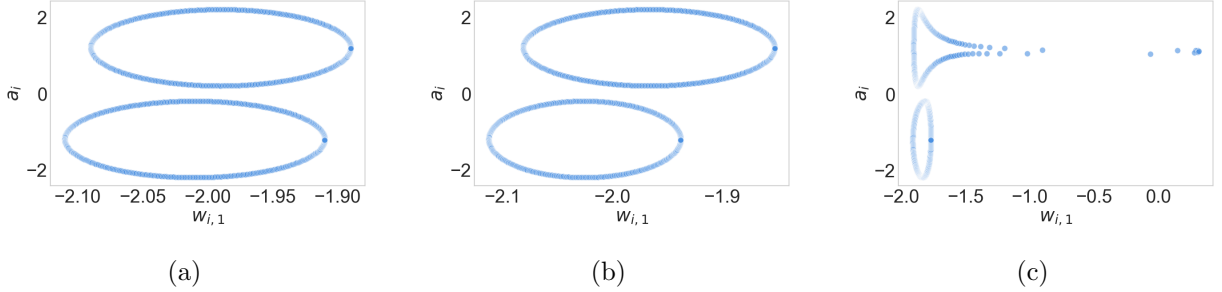
Figure 9: Topology of a 2D neural network with Adam. The neurons are initialized on the disjoint union of two genus-1 surfaces and optimized with Adam.
