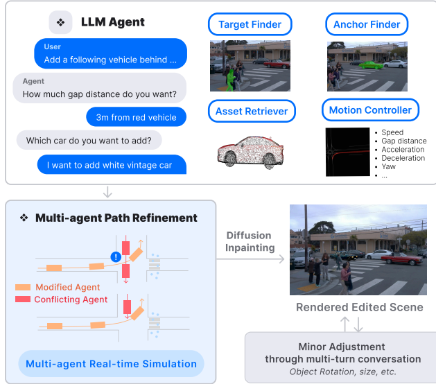
Figure 3. Editing process. Given a user prompt, the LLM agent coordinates multiple modules. After identifying the target object, retrieving assets, and planning an initial trajectory, the results are refined by the multi-agent path refinement module. Finally, diffusion-based inpainting is applied and the edited scene is rendered.
