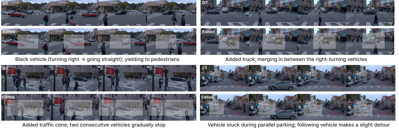
Figure 6. Qualitative results with predictive path refinement. The multi-agent path refinement module adapts both target and surrounding objects to interact in edited scenes. Gray areas indicate the edited regions, and images are zoomed in for clearer visualization.
