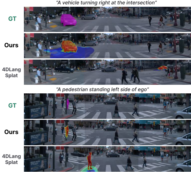
Figure 4. Qualitative comparison of object querying. Our method effectively captures the behaviors of road agents within the scene.
