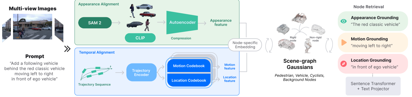
Figure 2. Pipeline of language alignment. The appearance and temporal alignment modules extract appearance, motion, and location features, which are then embedded into scene-graph Gaussians. Given a natural language prompt, these features enable grounding of the corresponding objects in the road scene.
