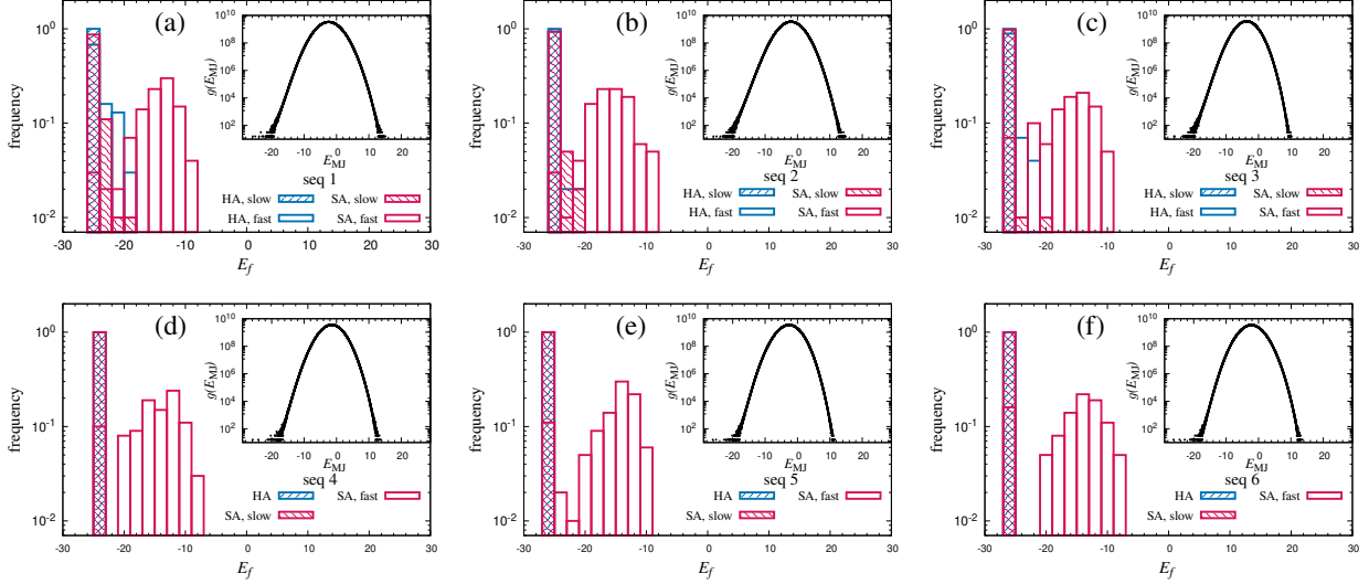
FIG. 3. Histograms of the final energy E_f [Eq. (2)] on a log scale for HA and SA computations for the six sequences in Table I, for the shortest (fast) and longest (slow) run times used. The insets show the density of states (log scale) calculated as a function of E_{MJ} . (a) Sequence 1. (b) Sequence 2. (c) Sequence 3. (d) Sequence 4. (e) Sequence 5. (f) Sequence 6.
