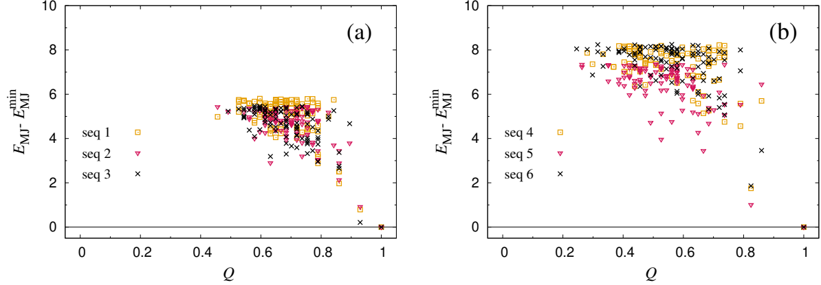
FIG. 4. Energy landscapes showing E_{MJ} - E_{MJ}^{\min} against the overlap Q with the native state for the 100 lowest-lying maximally compact states for each of the six sequences in Table I, as obtained through exhaustive enumeration (Sec. IIF, Appendix B). The overlap, or nativeness, Q of a structure is the fraction of ground state contacts it contains. (a) Sequences 1–3, with low-complexity topology A as their native state. (b) Sequences 4–6, with high-complexity topology B as their native state.
