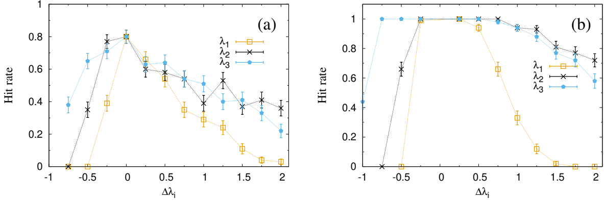
FIG. 5. Parameter dependence of the fraction of correct solutions (hit rate) in the vicinity of the best Lagrange parameters found, \boldsymbol{\lambda}^* = (1.5, 2.0, 2.0) , when using QUBO SA and QUBO HA to search for the ground state of sequence 5 (Table 1 in the main text). The hit rate is plotted against \Delta\lambda_i = \lambda_i - \lambda_i^* , keeping \lambda_j = \lambda_j^* for j \neq i . Each data point represents an average over 100 runs. The SA runs comprised 10,000 sweeps per temperature, while the HA run time was 10 s. Lines are drawn to guide the eye. (a) SA (b) HA.
