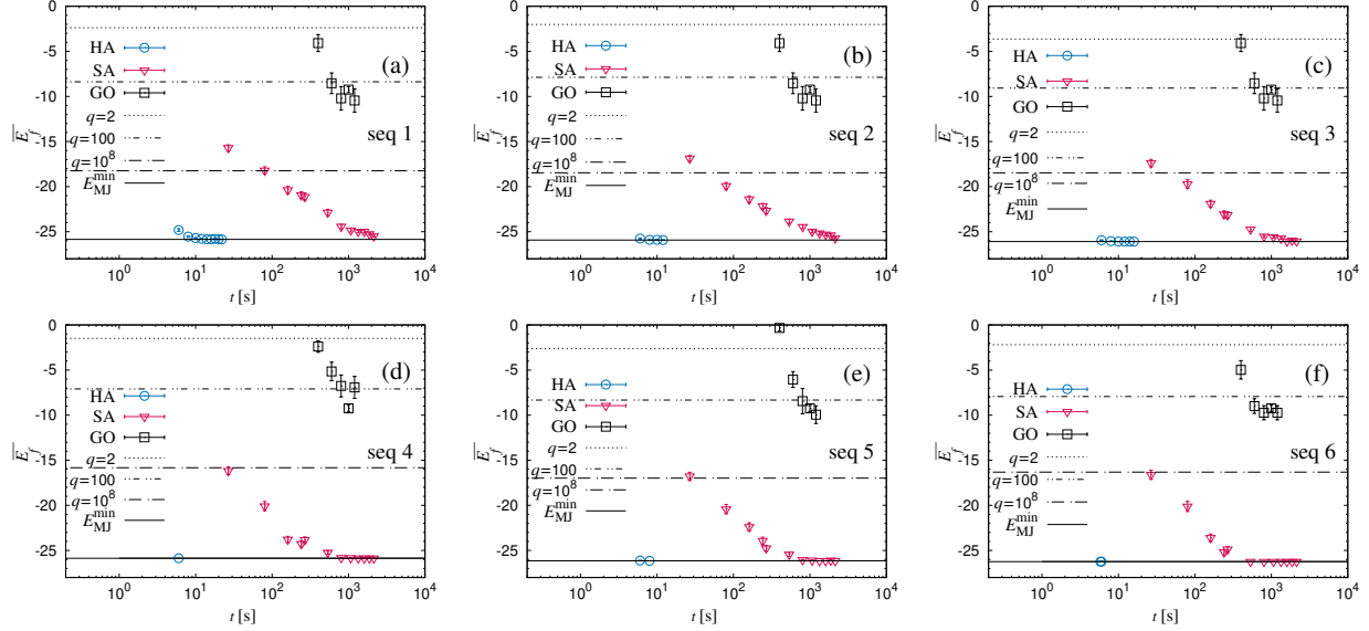
FIG. 2. Average final energy, \overline{E_f} , plotted against run time, t , in HA, SA and GO computations for the six sequences in Table I, with Lagrange parameters \lambda = (1.5, 2.0, 2.0) [Eq. (2)]. Each data point represent an average over 10 (GO) or 100 (HA and SA) independent runs. The horizontal lines indicate data on the distribution of E_{MJ} over valid chain structures, as obtained by exhaustive enumerations (Sec. II F). The lowest line represents E_{MJ}^{\min} . The other three represent the lowest q -quantiles for q = 2 (median), q = 100 and q = 10^8 , respectively. (a) Sequence 1. (b) Sequence 2. (c) Sequence 3. (d) Sequence 4. (e) Sequence 5. (f) Sequence 6.
