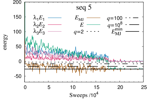
FIG. 1. Run-time evolution of the interaction potential E_{\text{MJ}} and the penalty energies E_1 , E_2 and E_3 [Eqs. (3–6)] in an SA run for sequence 5 (Table I), using \lambda = (1.5, 2.0, 2.0) , 25 temperatures and 10,000 sweeps at each temperature. The horizontal lines indicate data on the distribution of E_{\text{MJ}} over valid chain structures, as obtained by exhaustive enumerations (Sec. II F). The lowest line represents the minimum E_{\text{MJ}} , E_{\text{MJ}}^{\text{min}} . The other three lines represent the lowest q -quantiles for q = 2 (median), q = 100 and q = 10^8 , respectively.
