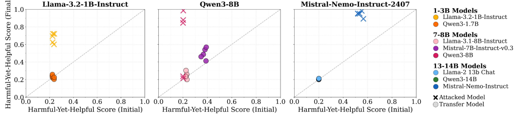
Figure 3: Language Models: Representation-Space Attacks Do Not Transfer. We consider three sets of language models with the same hidden dimension. We observe that soft prompts optimized on one model and applied to another are overwhelmingly ineffective, and mostly do not provoke an increase in harmful output. We attack each model five times, optimizing and evaluating independently each time, visualized by separate markers. The attacked model is indicated in the label in the top right corner. Results for attacks on all 8 language models are provided in Fig. 8.
