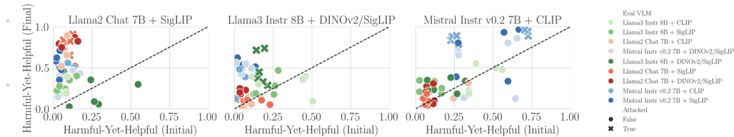
Figure 6: Vision-Language Models: Representation-Space Attacks Can Transfer if Optimized at a Precise Layer. Optimizing jailbreaks on the post-projector latent representation of a model permits attack transfer to target models.
