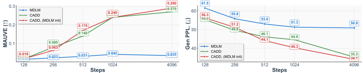
Figure 5 Analogous figure of Figure 4. We compare the finetuned checkpoint using CADD objective with CADD and the initialization checkpoint of MDLM.
