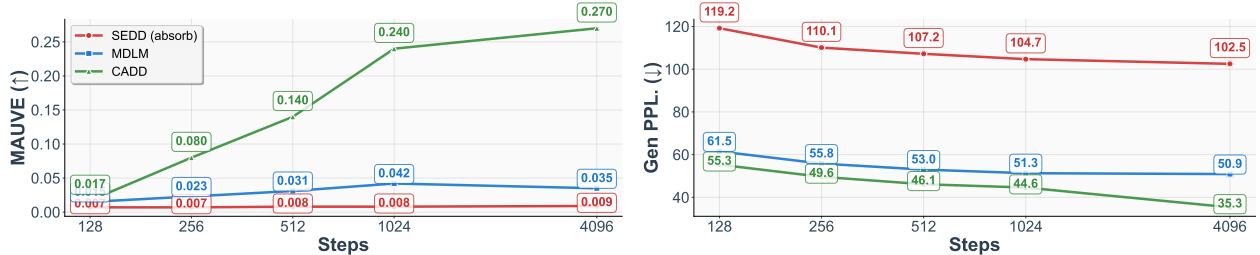
Figure 4 Unconditional text generative evaluation of model trained on OpenWebText (OWT) data. All method are evaluated with 128, 256, 512 1024, and 4096 sampling steps. MAUVE ( Left Panel , higher is better) and generative perplexity ( Right Panel , measured using GPT2-Large, lower is better) are reported.
