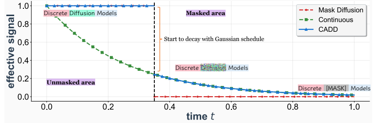
Figure 2 Example of Signal-to-Noise Ratio (SNR) change of one token in the forward of vanilla Mask Diffusion vs. CADD ( Best view in color ). After the second token is masked at the first time, CADD gradually corrupt the information of this token with Gaussian diffusion in the latents, resulting in a smooth decay.
