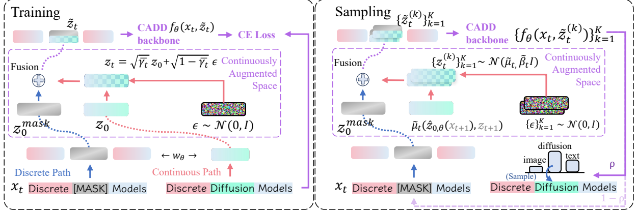
Figure 3 (Best view in color) Illustrative depiction of CADD model, combining both the discrete and continuous feature of the data. In training, the clean token at the masked position will be created by embedding matrix and used to form the noisy embedding according to the continuous forward. In sampling, the model is able to predict a diverse distribution of possible tokens by sampling multiple z_t . Then the predicted tokens will be recycled into the embedding matrix to form \hat{z}_{0,\theta} for the next iteration.
