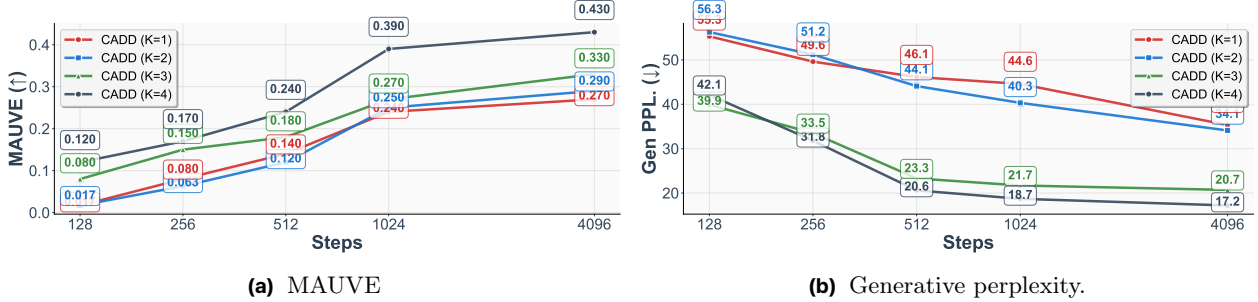
Figure 6 Analogous figure of Figure 4, comparing CADD variants using K=1-4 to estimate \hat{x}_0 .
