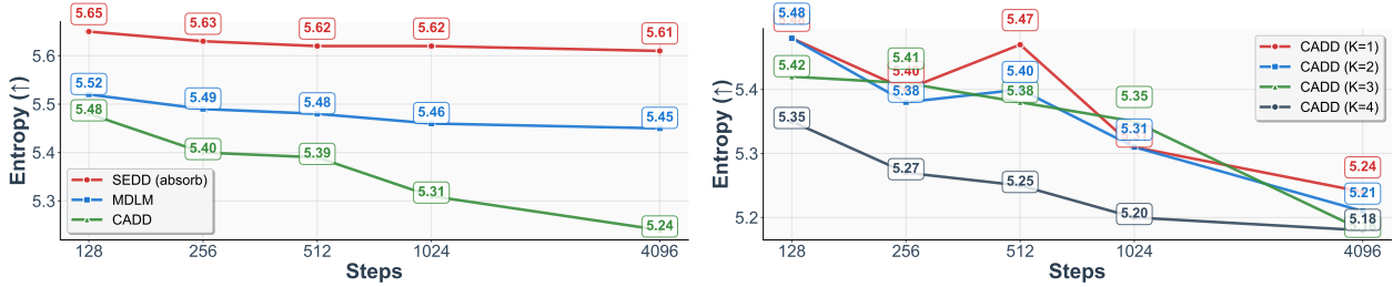
Figure 7 Analogous figure of Figure 4: study of generation variance and diversity across all methods and across different K . We use entropy (higher indicates more stochasticity) are reported.
