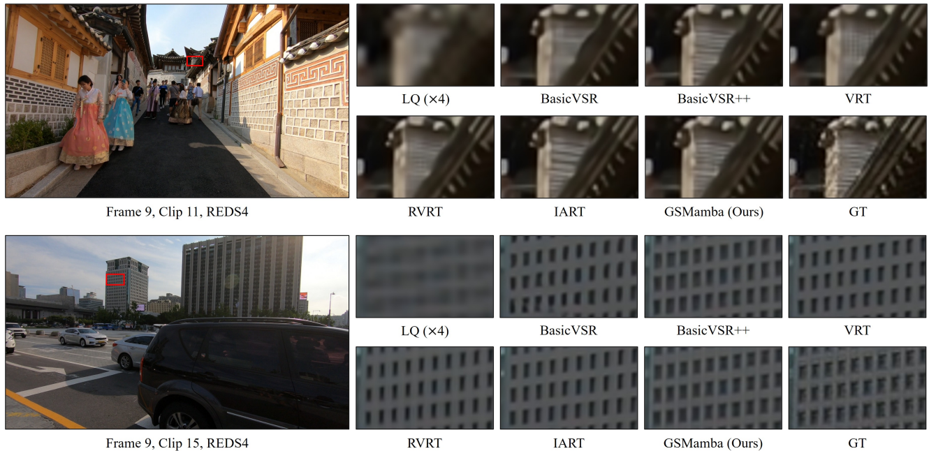
Figure 5. Qualitative results with the state-of-the-art methods on REDS4 [29] dataset
