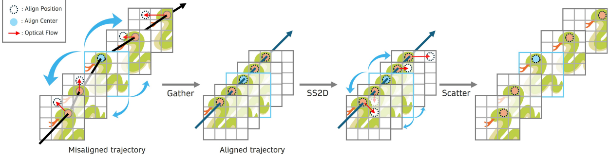
Figure 2. Overview of the proposed Gather-Scatter mechanism. Misaligned trajectories across frames are first temporally aligned toward the anchor frame (align center) using optical flow (Gather). The aligned features are then flattened in temporal-first order and processed by SS2D (Mamba) for long-range temporal modeling. Finally, the output residuals are inversely warped back to their original frame positions (Scatter), updating all frames within the window.
