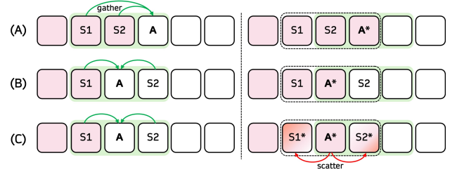
Figure 3. Comparison of windowed propagation strategies. (A) Forward-anchored propagation : supporting frames S1 , S2 are aligned toward the anchor A located at the end of the window, and only the anchor is updated. (B) Center-anchored propagation : supporting frames are aligned toward the anchor placed at the center of the window, reducing alignment path length and improving feature aggregation. (C) Center-anchored + Scatter (ours) : residuals aligned at the center are redistributed back to all supporting frames, enabling joint enhancement of the entire window.
