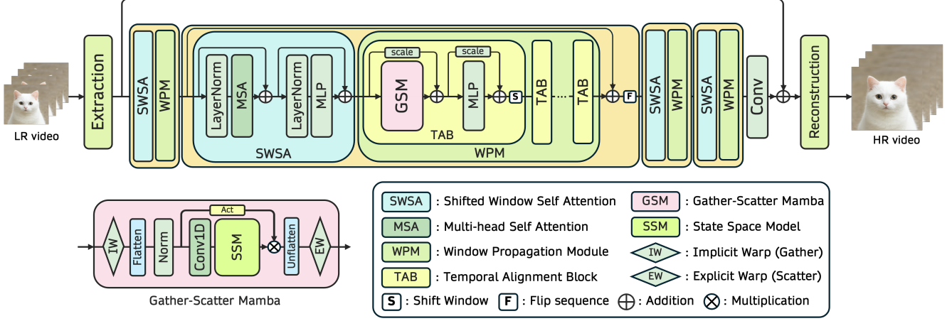
Figure 1. Overall architecture of the proposed Gather-Scatter Mamba (GSM). Given a low-resolution input sequence, local spatial refinement is first performed using shifted window self-attention (SWSA). Temporal propagation is then carried out by the window propagation module (WPM). Within each WPM, the GSM block first gathers features by aligning all frames to an anchor frame, processes the aligned features using Mamba’s directionally selective scanning, and then scatters the updated features back to their original temporal locations.
