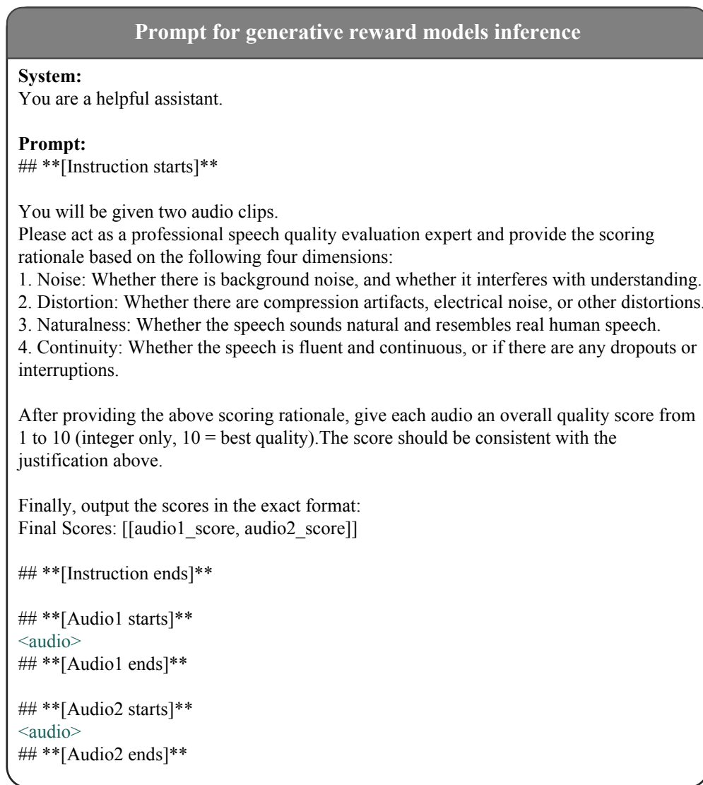
Figure 8: Prompt structure for generative reward models inference.
