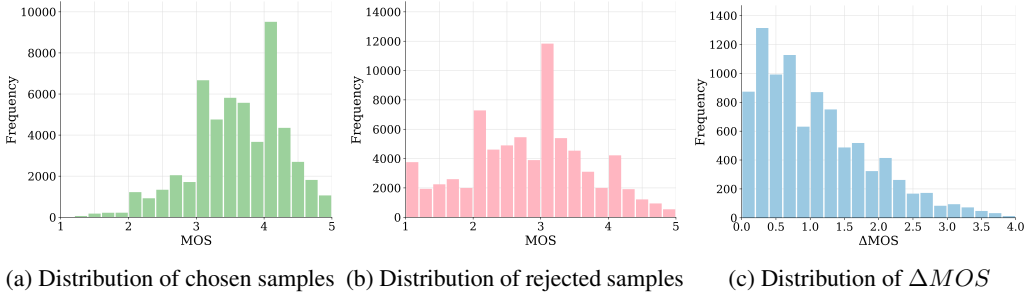
Figure 2: Distribution of MOS scores in MOS-RMBench. Figures (a) and (b) show the MOS distributions of chosen and rejected samples. Figure (c) presents the distribution of \Delta MOS in the test set.
