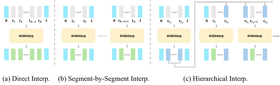
Figure 3: Comparison of interpolation strategies in ArbInterp. ArbInterp supports multiple interpolation strategies: (a) Direct Interpolation for short-range interpolation, and two for long-term scenarios: (b) Segment-by-Segment Interpolation and (c) Hierarchical Interpolation .
