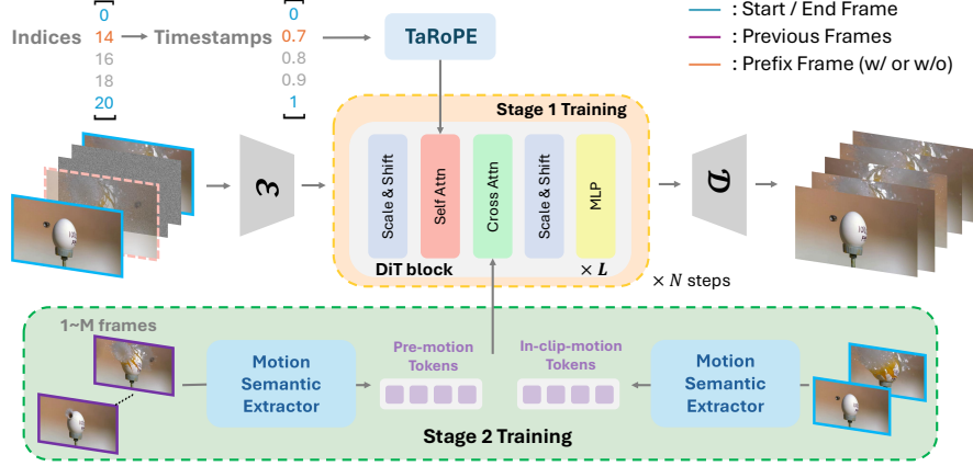
Figure 2: Overall architecture of ArbInterp. Our framework enables arbitrary-length interpolation with continuous timestamps using Timestamp-aware Rotary Position Embedding (TaRoPE) . Additionally, we introduce an appearance-motion decoupling conditioning strategy to enhance the performance of long-term interpolation. This strategy ensures appearance consistency via prefix frame guidance and enforces motion continuity through motion tokens.
