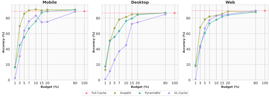
Figure 2: Performance comparison of KV cache methods on ScreenSpotV2. SnapKV’s uniform allocation outperforms approaches that allocate varying budgets.
