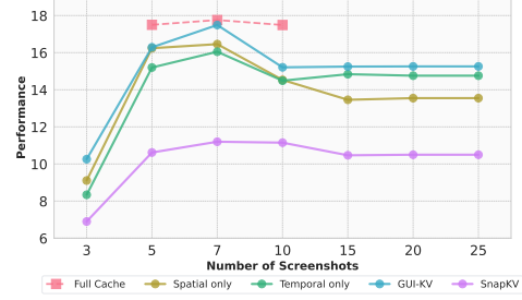
Figure 4: Ablation studies on AgentNetBench with various number of screenshots.
