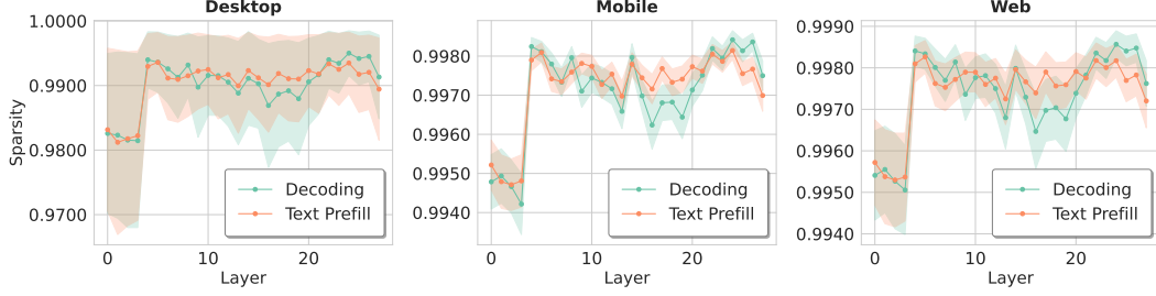
Figure 1: Attention sparsity for UI-TARS-1.5-7B across layers for screenshots from ScreenSpot-V2. All scenarios exhibit extremely high sparsity (mostly > 0.99 ) across all layers.
