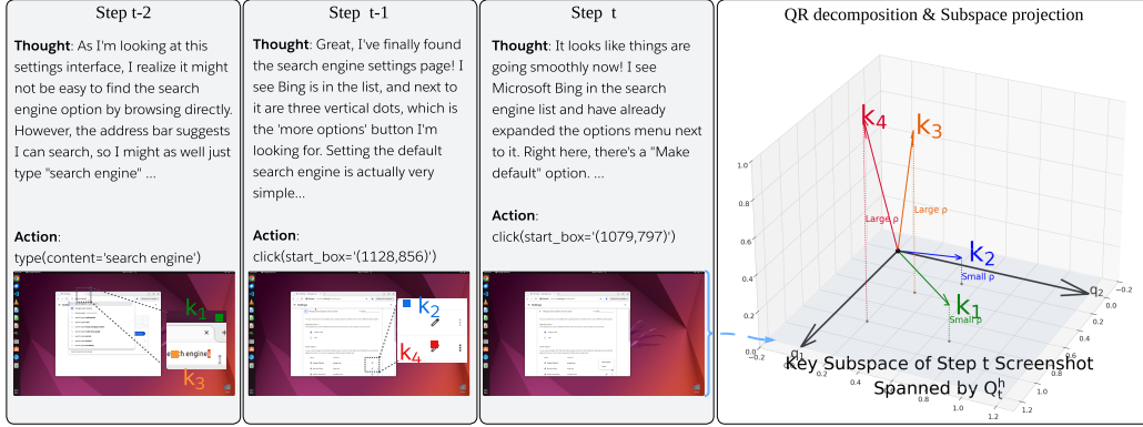
Figure 3: Illustration of our temporal redundancy scoring mechanism. We first perform QR decomposition on the current screenshot at step t to obtain a subspace spanned by Q_t^h . Then, we project key vectors k_i^h s of visual tokens from previous frames onto Q_t^h . The magnitude of the residual \rho (the component orthogonal to the subspace) quantifies the visual token’s non-redundancy. In this example, k_3 and k_4 are less redundant than k_1 and k_2 since they have larger residuals orthogonal to Q_t^h .
