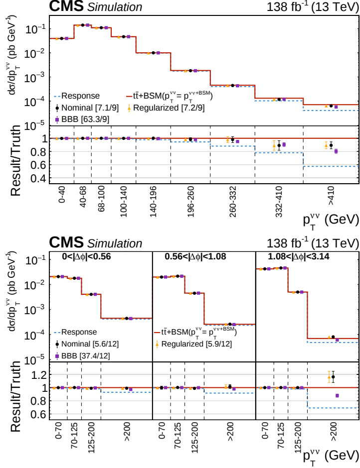
Figure 6: Result of the closure test based on simulation accounting for potential BSM contributions based on a top squark pair production scenario with a stop mass of 525 GeV and a neutralino mass of 350 GeV. The potential BSM contribution is scaled by a factor of ten. The test is performed for the p_T^{VV} (upper) and 2D measurement (lower) using the nominal (black circles), the regularized (orange triangles), and the bin-by-bin unfolding (purple squares), based on all data-taking periods combined. The unfolded distributions are compared to the expected distribution (red solid line) based on the sum of the nominal dileptonic t\bar{t} signal sample and BSM signal with the corresponding \chi^2 / (\text{number of degrees of freedom}) values given in the legend in square brackets. The distribution used for the response matrix is shown in blue (dotted line). The error bars correspond to the statistical uncertainty. The lower part shows the ratios between the unfolded and the expected distributions.
