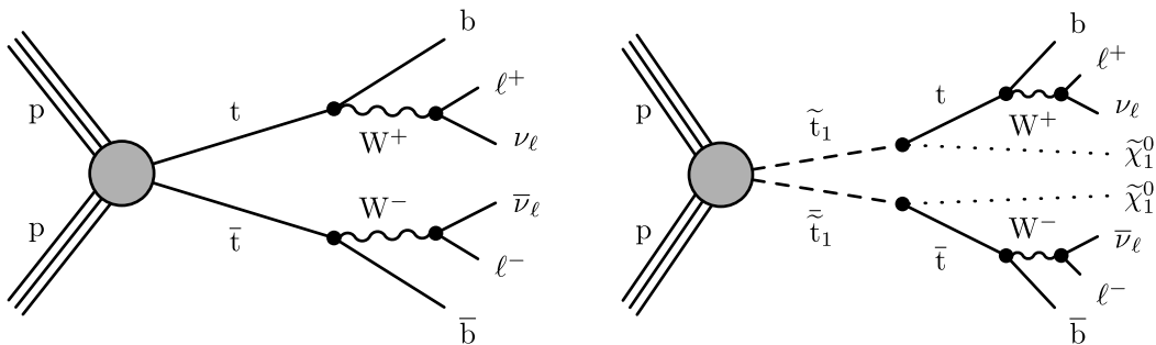
Figure 1: In the left diagram, the SM t\bar{t} production process is sketched, whereas the right diagram shows the production of a hypothetical top squark pair, \tilde{t}_1\tilde{t}_1^* , with both top squarks decaying to a top quark and a neutralino, \tilde{\chi}_1^0 . This analysis focuses on signatures, where both of the W bosons decay leptonically.
