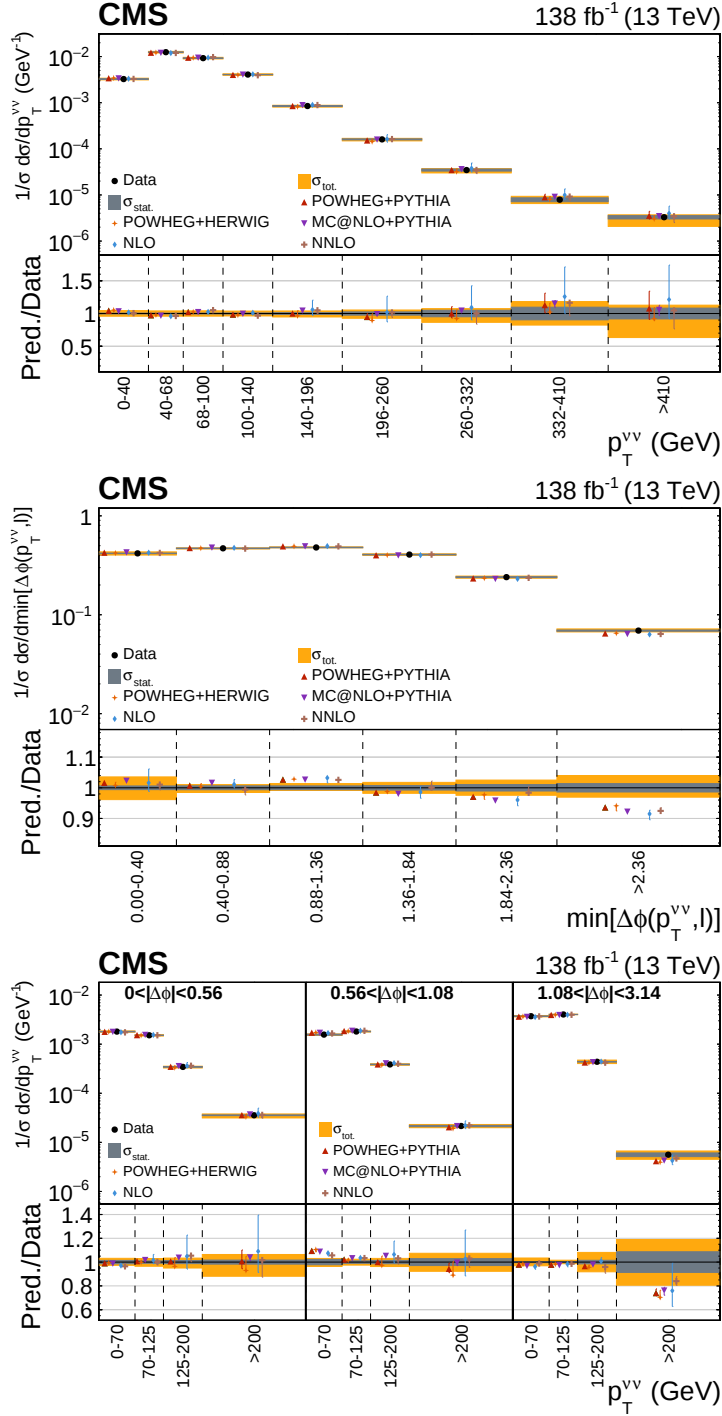
Figure 8: The measured normalized differential signal cross sections (black markers) as functions of p_T^{\nu\nu} (upper), \min[\Delta\phi(\vec{p}_T^{\nu\nu}, \vec{p}_T^\ell)] (middle), and double-differential in both observables (lower) are shown. The theoretical predictions from POWHEG+PYTHIA (dark red), POWHEG+HERWIG (orange), MC@NLO+PYTHIA (purple), and the fixed-order NLO (light blue) and NNLO (brown) calculations are compared to the measurement. The cross sections in the last p_T^{\nu\nu} bin of the upper (lower) plot are determined for p_T^{\nu\nu} > 410 (200) GeV and normalised to a bin width of 90 (200) GeV for visualisation purposes. The total (statistical) uncertainty on the measurement is shown as an orange (dark grey) band. The lower panel of each plot shows the ratio between theoretical predictions and the measurement.
