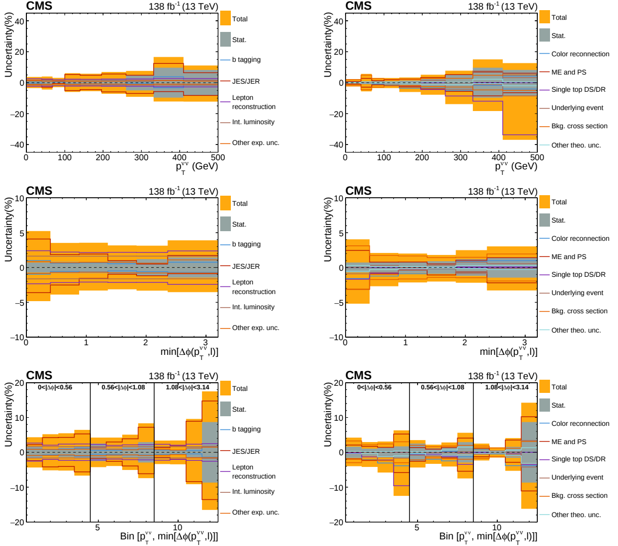
Figure 4: Breakdown of the relative uncertainties from experimental (left) and theoretical (right) uncertainties on the differential cross section measurement as a function of p_T^{vv} (upper), \min[\Delta\phi(\vec{p}_T^{vv}, \vec{p}_T^\ell)] (middle), and both variables (lower). In the last case, each group of four bins corresponds to p_T^{vv} bins, and \min[\Delta\phi(\vec{p}_T^{vv}, \vec{p}_T^\ell)] bin edges are indicated by vertical solid lines. The statistical uncertainty (dark grey) takes the size of available event counts in both the simulated samples and the recorded data into account. The last bin includes all events above the plotted range.
