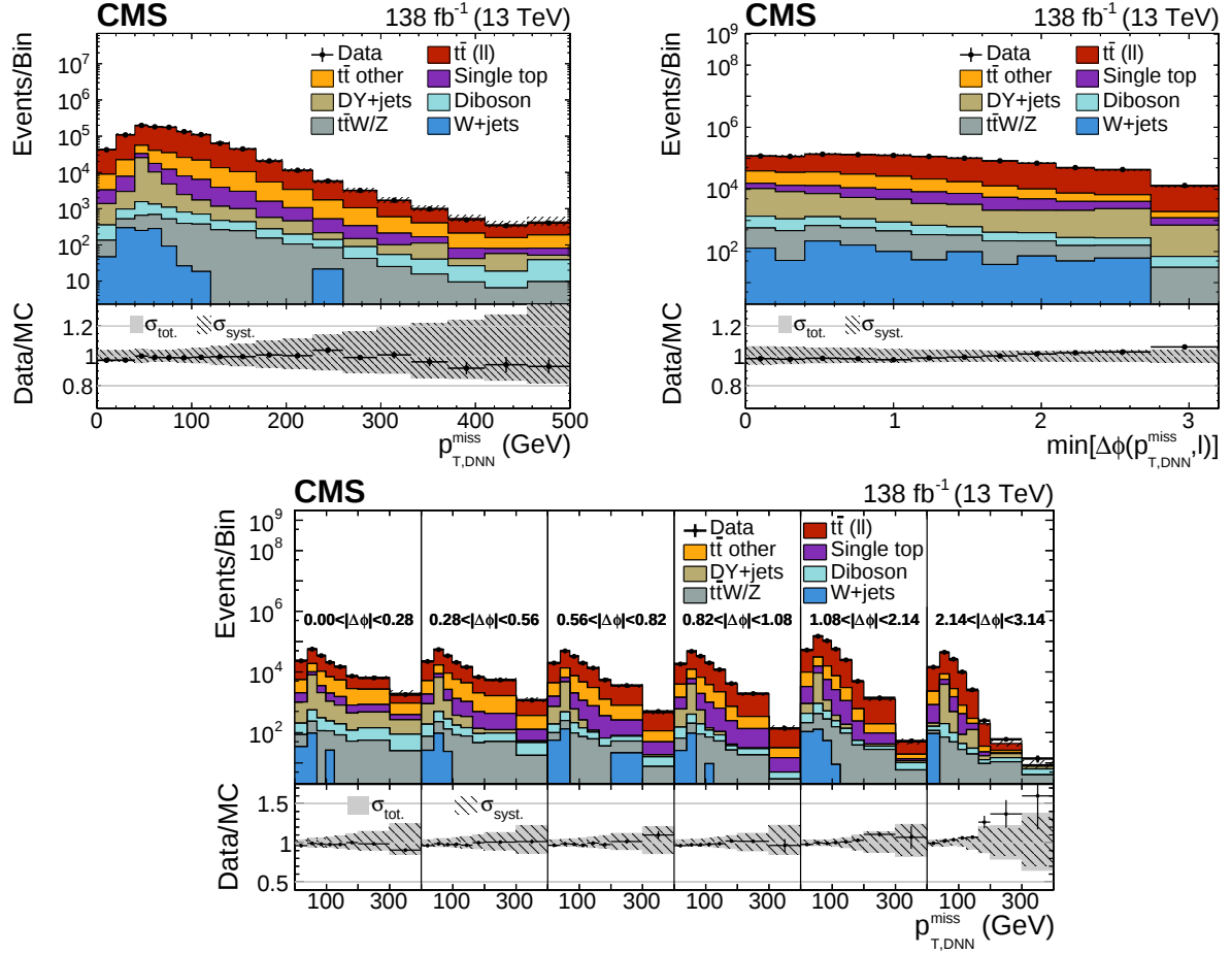
Figure 5: The observed (black markers) and simulated distributions of p_{T,DNN}^{\text{miss}} (upper left), \min[\Delta\phi(\vec{p}_{T,DNN}^{\text{miss}}, \vec{p}_T^\ell)] (upper right), and the 2D distribution (lower) with both observables are shown. Events from all data-taking periods and all channels are combined. The hatched (grey) areas indicate the systematic (total) uncertainty on the simulation. Vertical and horizontal error bars on the data points represent the statistical uncertainty and the bin width, respectively. The lower panel of each plot shows the ratio of observed data to the expectation from MC simulation in each bin. The last bin includes all events above the plotted range.
