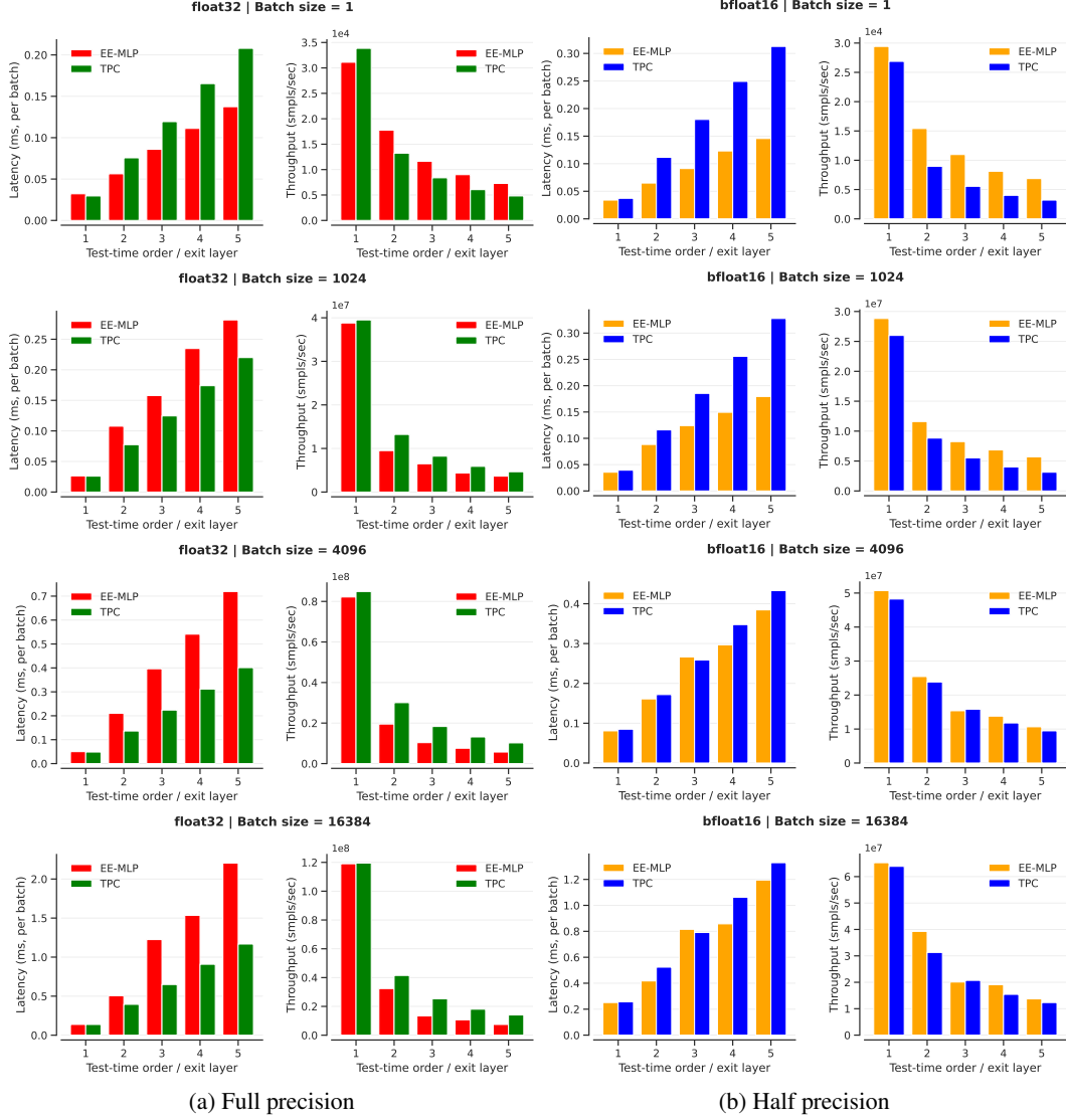
Figure 12: Inference time costs (latency and throughput) for varying batch sizes: EE-MLPs are faster than TPCs at small batch sizes. However, for medium-large batch sizes, TPCs have similar speeds at half precision and we find them to be even faster at full precision.
