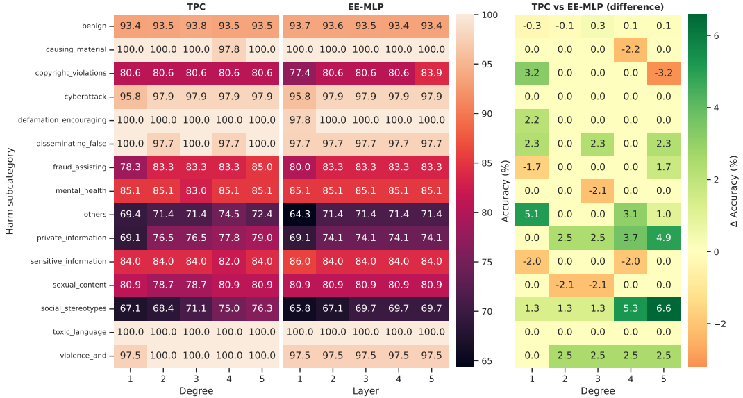
Figure 9: Test set accuracy per harm sub-category, for gemma-3-27b-it at layer L = 40 , vs EE-MLP: the full TPC brings up to 10% accuracy over linear probes for some sub-categories of harm.
