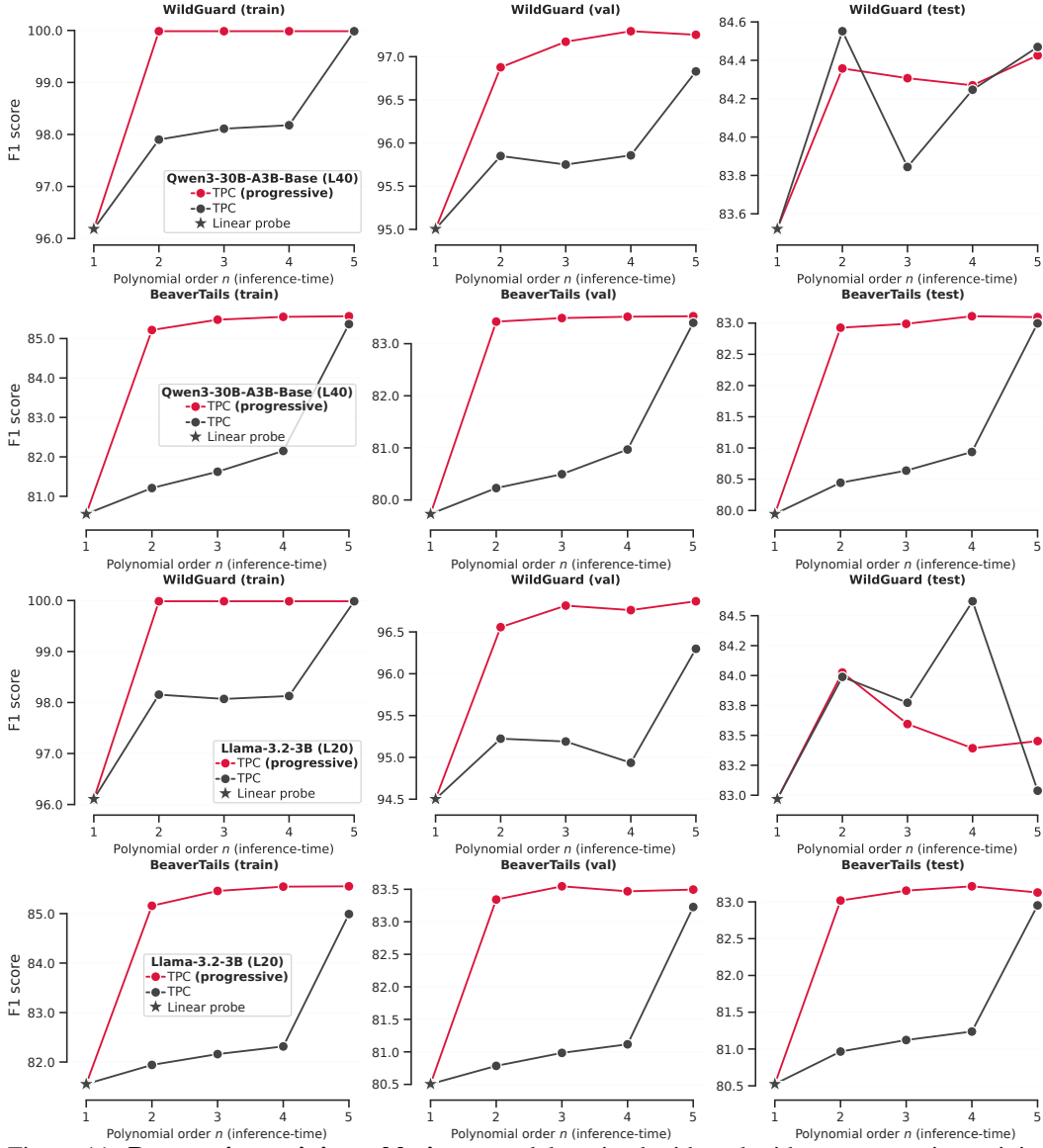
Figure 11: Progressive training, ablations: models trained with and without progressive training on Qwen3-30B-A3B-Base and Llama-3.2-3B models.
