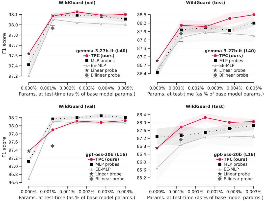
Figure 2: Results on WildGuardMix (gemma-3, gpt-oss): F1 score on harmful prompt classification for probes evaluated with increasing compute at inference-time (full results in Section F).
