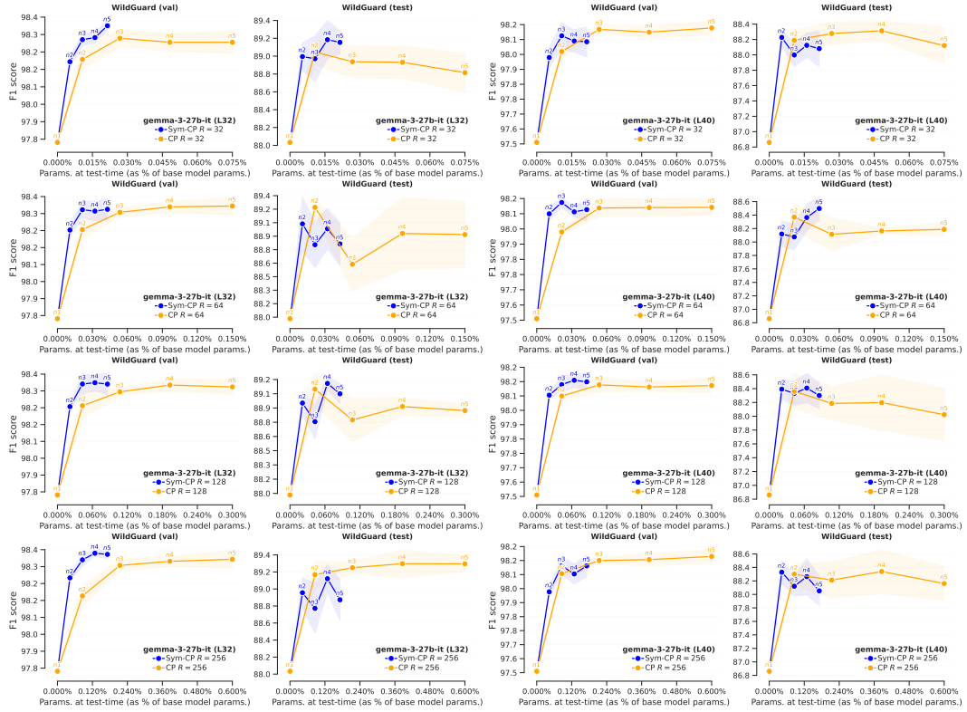
Figure 16: Ablation (symmetric vs non-symmetric CP): F1 score on harmful prompt classification for probes evaluated with increasing compute at test-time, for the two parameterizations on WildGuardMix. Across ranks \{32, 64, 128, 256\} the symmetric CP maintains similar performance to the unconstrained CP, with a fraction of the parameter count.
