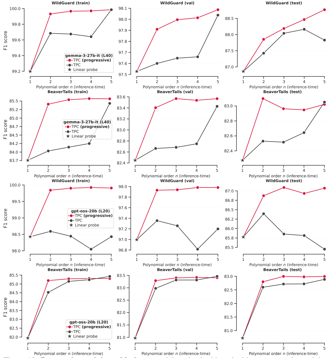
Figure 10: Progressive training, ablations: models trained with and without progressive training on gemma-3-27b and gpt-oss-20b models.
