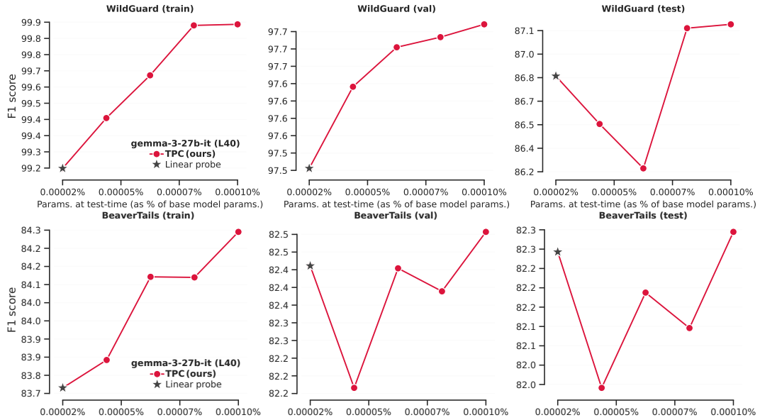
Figure 15: Rank R = 1 ablation : we find that using the smallest possible rank leads to models often struggling to reliably improve over linear probes. We suggest a minimum rank of \sim 32 when training TPCs.
