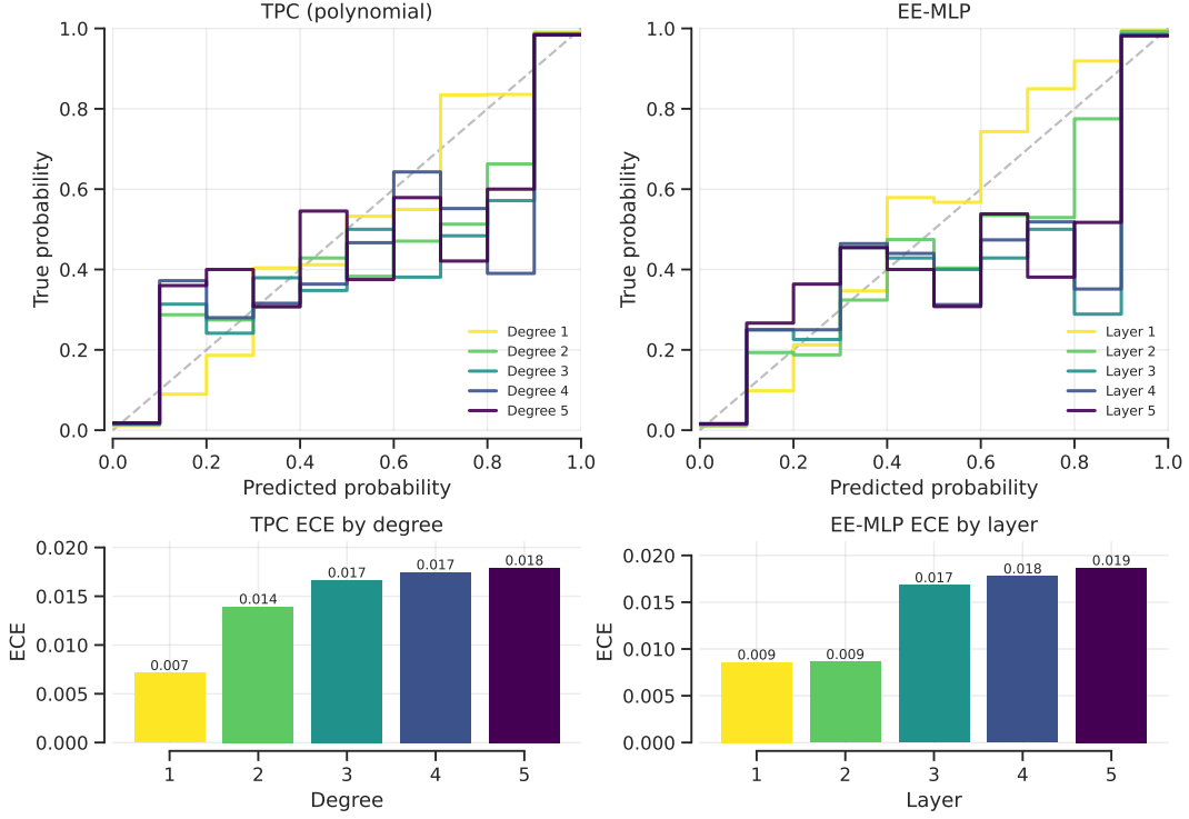
Figure 8: Calibration plots: both dynamic models are relatively well calibrated.
