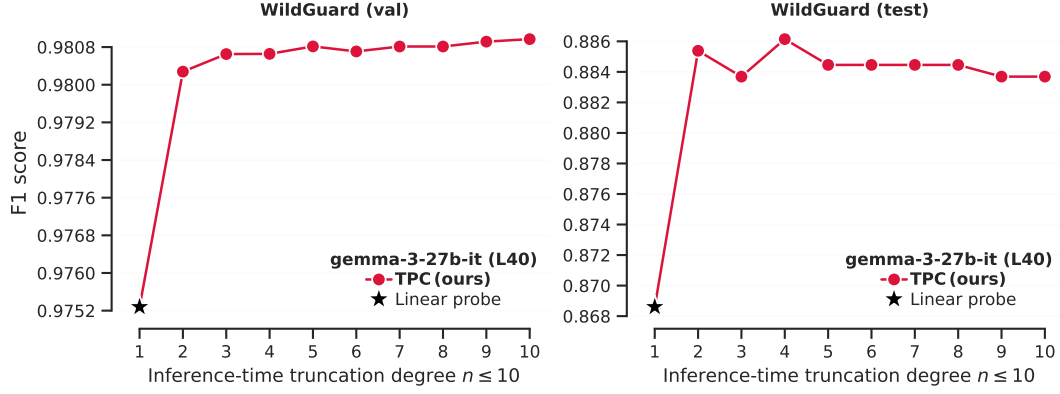
Figure 14: Ablation (maximum degree N ) : training a single high-degree N = 10 polynomial (with the default R = 64 ); we find diminishing returns from very high-degree terms.
