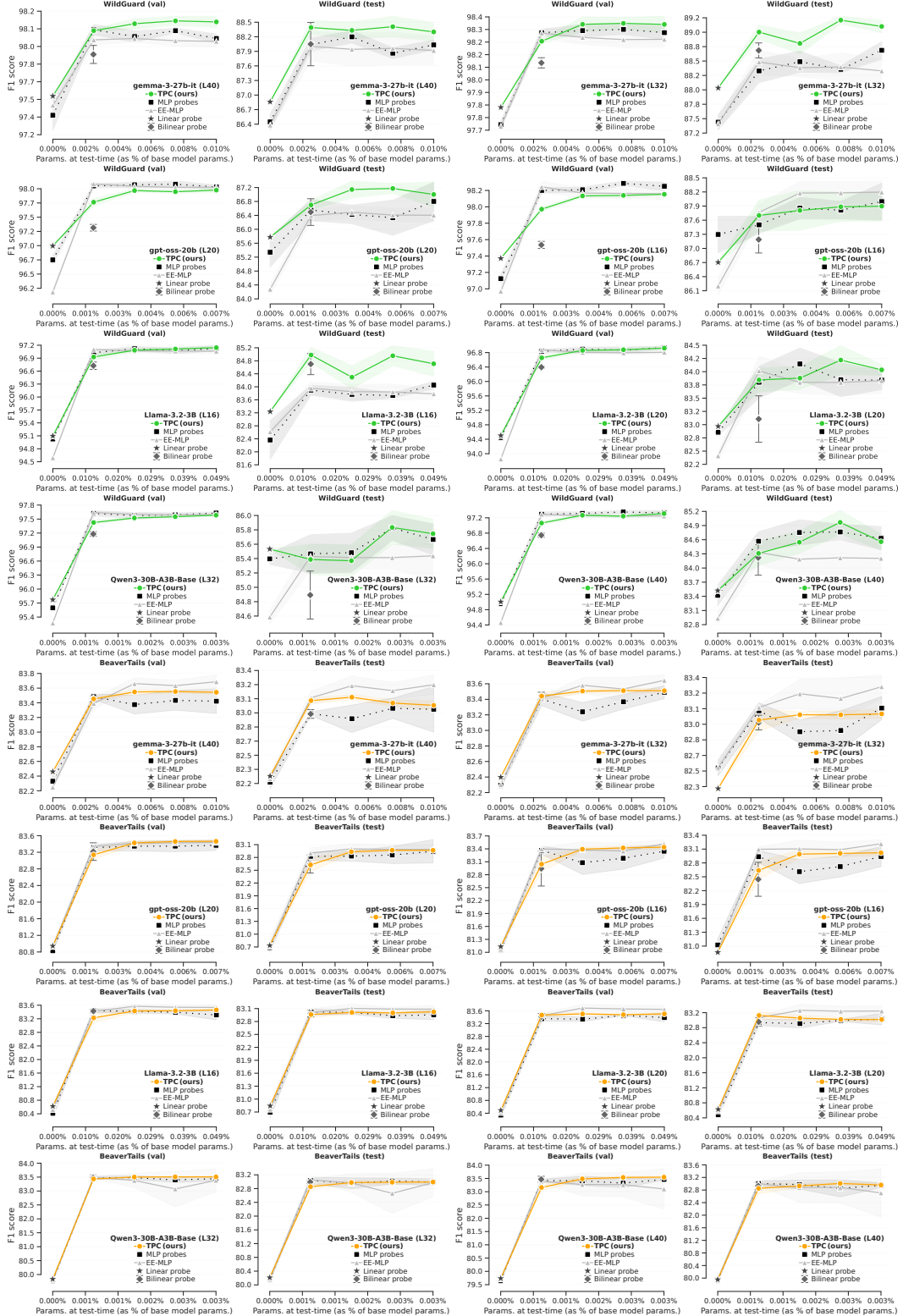
Figure 18: Full baseline comparisons on WildGuardMix and BeaverTails for rank R = 128 : F1 score on harmful prompt classification for probes evaluated with increasing compute at test-time. All baselines are parameter-matched to TPCs, and have dedicated hyperparameter sweeps.
