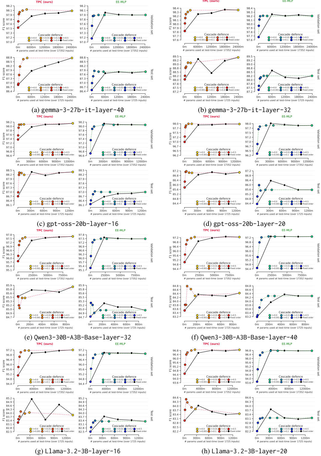
Figure 7: Full baseline comparisons on WildGuardMix: Cascaded evaluation for TPCs vs early-exit MLPs.
