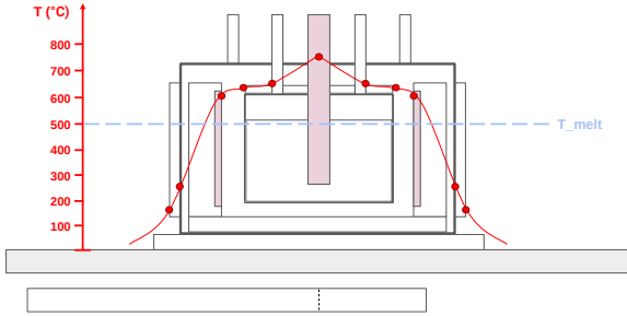
(b) Approximate typical steady-state radial distribution of temperature, showing that the full salt volume is above the melting temperature of CILiF.
