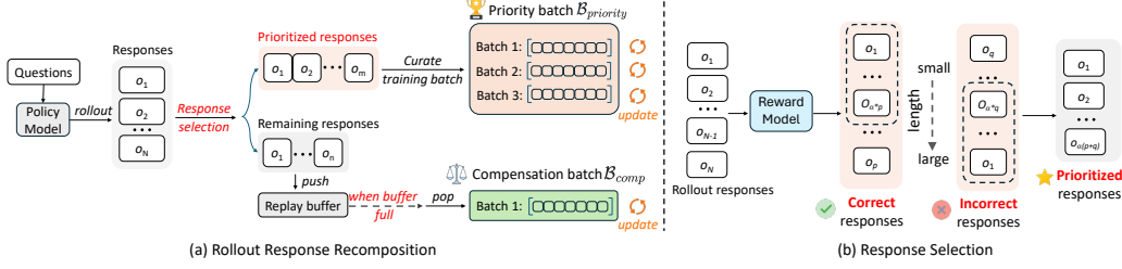
Figure 2: (a) The overall framework of RoRecomp. After the response generation, we recompose candidate responses into two types of batches: priority batches and compensation batches. (b) The details of response selection. We select prioritized responses for each question by jointly considering the response length and reward.
