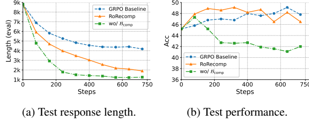
Figure 4: Effectiveness of compensation batches, with response length and performance averaged across six math test sets and reported at various training steps.
