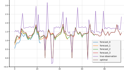
(b) 192-prediction on the Electricity dataset
