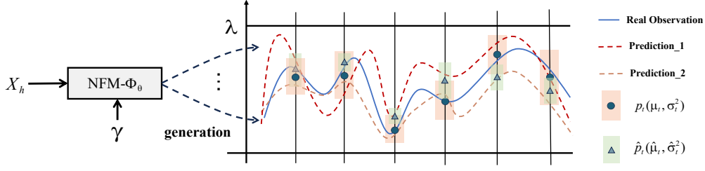
Figure 1: Illustration of the MNFP.
