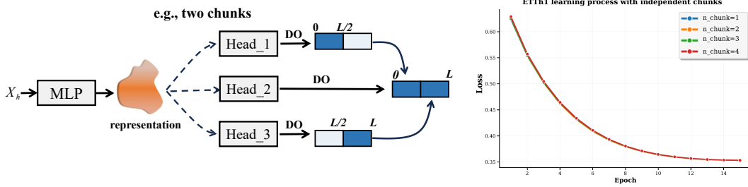
Figure 3: We make the forecast by applying independent heads on several non-overlapped chunks. The right figure shows the learning process in different settings.
