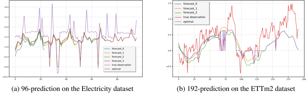
Figure 9: Visualization of forecasting results of ReNF. The figure shows multiple outputs of ReNF in different layers, along with the result of applying optimal post-combination.
