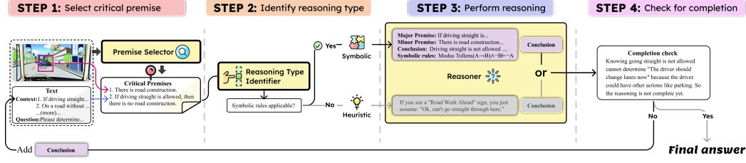
Figure 4: LogiCAM Workflow. The figure illustrates a single iteration; the complete multi-iteration reasoning process is detailed in Section 9.
