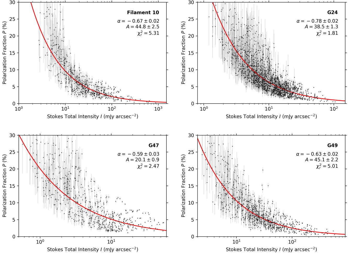
Figure 17. Debiased polarization fraction P as a function of the Stokes I total intensity for the vectors plotted in Figure 8 through 11. The intensity I is shown on a logarithmic scale to better visualize the spread of P for lower values of I . The best fit to the power law given in Equation 9 is shown as a red plain line for each bone, and the associated parameters A and \alpha are provided directly on the plot. Only every fourth vector is plotted and used for the fit, and the uncertainty in P is shown as gray lines. Continued from Figure 16.
