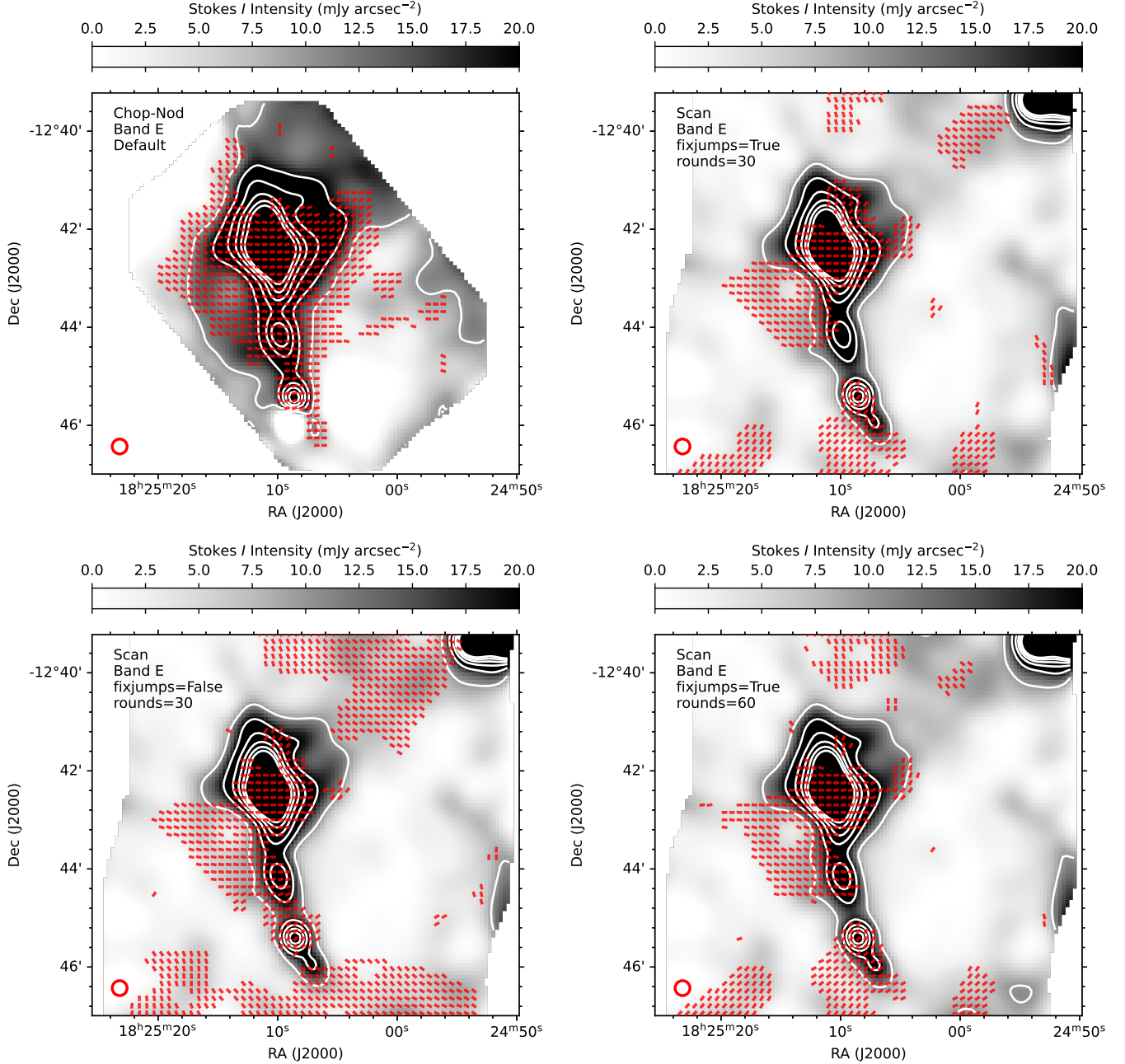
Figure 18. The magnetic field structure (red single-length vectors) inferred from HAWC+ 214 \mu\text{m} (Band E) observations for four different data reduction procedures for Filament 5. Every other vector is plotted. The gray scale is the measured 214 \mu\text{m} Stokes I total intensity, and the white contours trace levels of 10 to 60 mJy arcsec ^{-2} by steps of 10 mJy arcsec ^{-2} . The red circle shows the beam of HAWC+ at 214 \mu\text{m} . Top left: Chop-Nod data reduced using the default pipeline parameters. Top right: Scan mode data reduced using \text{rounds}=30 and \text{fixjumps}=\text{True} (see also Figure 5 for full map). Bottom left: Scan mode data reduced using \text{rounds}=30 and \text{fixjumps}=\text{False} . Bottom right: Scan mode data reduced using \text{rounds}=60 and \text{fixjumps}=\text{True} .
