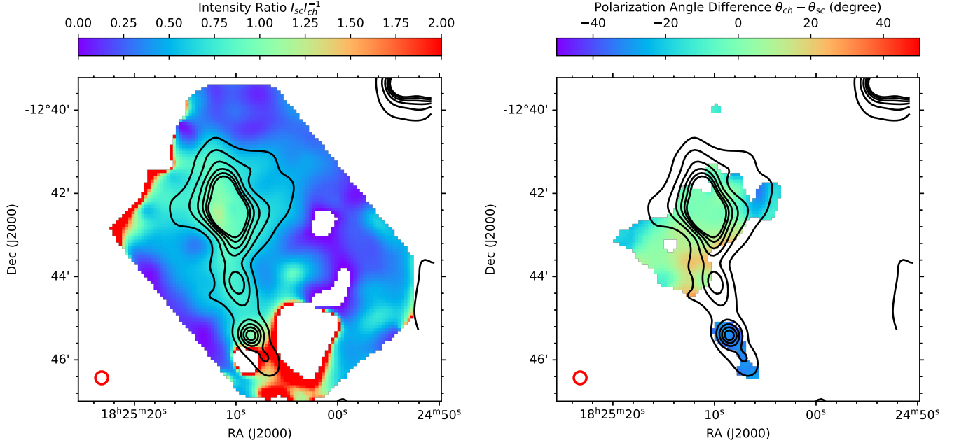
Figure 19. Comparison between Chop-Nod and Scan mode data for Filament 5. The Stokes I , Q , and U data from the Scan mode observations were re-gridded to match the Chop-Nod data. The black contours trace the Stokes I total intensity from the Scan mode map from 10 to 60 mJy arcsec ^{-1} by steps of 10 mJy arcsec ^{-1} . The HAWC+ beam is given as a red circle in each panel. Left: The intensity ratio I_{sc}I_{ch}^{-1} is shown on a rainbow scale for the pixels where I > 0 in both maps. Right: The difference of the polarization angles \theta_{ch} - \theta_{sc} is shown on a rainbow scale for the pixels where P/\delta_P > 3 , P < 30\% , and I/\delta_I > 10 in both maps.
