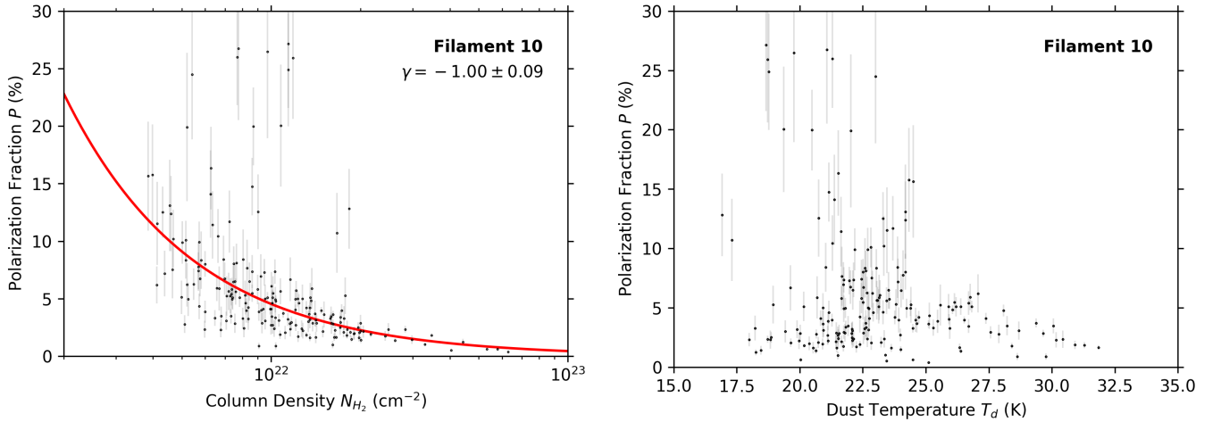
Figure 25. Polarization fraction P as a function of the gas column density N_{H_2} (left panel) and the dust temperature T_d (right panel) for Filament 10. The full red line traces a power-law fit of the form P \propto N_{H_2}^\gamma . The HAWC+ data was smoothed and re-projected to share the same resolution and pixel scale as the Herschel column density and temperature maps described in Section 2.2. Only every other vector from the resulting smoothed catalog is plotted and used for the fit, and the uncertainty in P is shown as gray lines.
