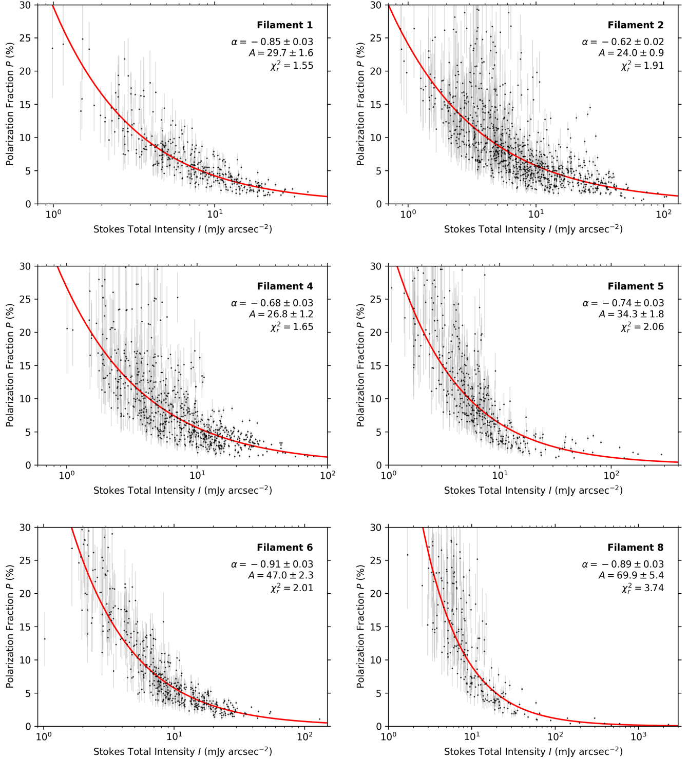
Figure 16. Debiased polarization fraction P as a function of the Stokes I total intensity for the vectors plotted in Figures 2 through 7. The intensity I is shown on a logarithmic scale to better visualize the spread of P for lower values of I . The best fit to the power law given in Equation 9 is shown as a red solid line for each bone, and the associated parameters A and \alpha are provided directly on the plot. Only every fourth vector is plotted and used for the fit, and the uncertainty in P is shown as gray lines. Continued in Figure 17.
