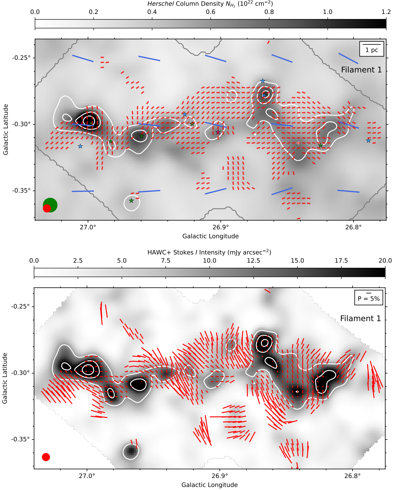
Figure 2. Filament 1. Top: The inferred magnetic field structure (HAWC+ 214 \mu\text{m} : red, Planck 850 \mu\text{m} : blue) plotted on the Herschel -derived N_{\text{H}_2} column density map (gray). The magnetic field angle \theta_B is obtained from rotating the polarization angle \theta by 90^\circ . Class I (green), Flat Spectrum (violet), and Class II (blue) YSOs are identified with star symbols. The gray contour denotes the area observed by HAWC+. The circles denote the beam sizes of HAWC+ (red) and Herschel (green). Bottom: The polarization measurements (red) plotted on the HAWC+ Stokes I total intensity map (gray) at 214 \mu\text{m} . The vector length shows the polarization fraction P . For each panel, only every third vector is plotted for both SOFIA and Planck data, and the white contours trace the Stokes I total intensity from 10 \text{ mJy arcsec}^{-2} and increasing by steps of 10 \text{ mJy arcsec}^{-2} . See Section 3.3 for details.
