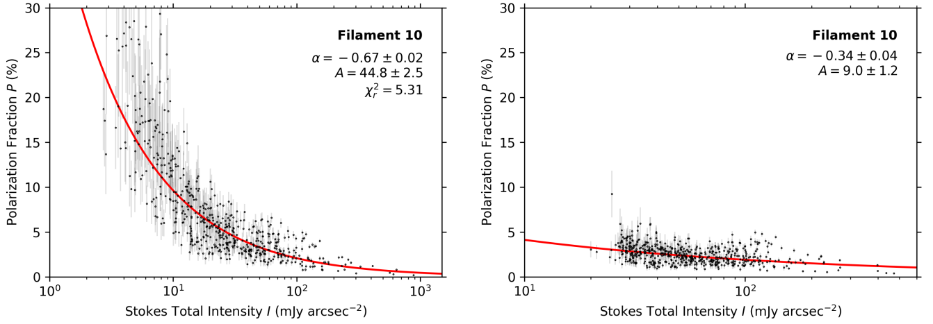
Figure 26. Polarization fraction P as a function of the Stokes I total intensity for Filament 10. The left panel shows the same relation as in Figure 17 as reference, while the right panel substitutes the Stokes I total intensity by the Herschel -derived flux densities at 214\ \mu\text{m} from Appendix F. In each panel, the data is fitted with a power law of the form P = AI^\alpha . Only every fourth vector is plotted and used for the fit, and the uncertainty in P is shown as gray lines.
