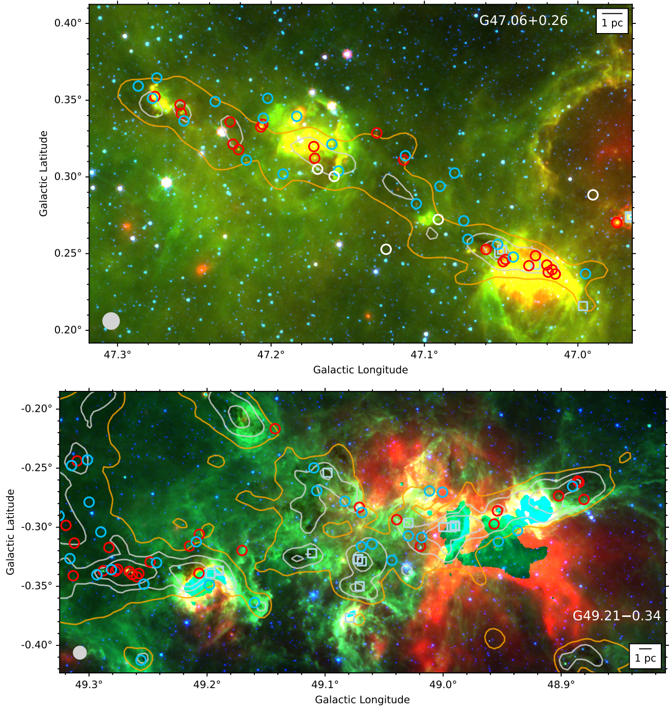
Figure 32. Spitzer red (24 \mu\text{m} ), green (8.0 \mu\text{m} ), and blue (3.6 \mu\text{m} ) composite image for G47 (top) and G49 (bottom). The color levels were chosen to highlight infrared-dark features, but we note that G49 is heavily saturated in these Spitzer bands. Class I and Flat Spectrum (red), Class II (blue), and Class III (white) YSOs from the literature are identified with circles. Masers are identified with squares when available. The three contours trace Herschel -derived N_{\text{H}_2} column densities of 0.5 , 1.0 , and 2.0 \times 10^{22} \text{ cm}^{-2} , with the lowest level identified in orange for clarity. The Herschel beam is given by the gray circle at the bottom left.
