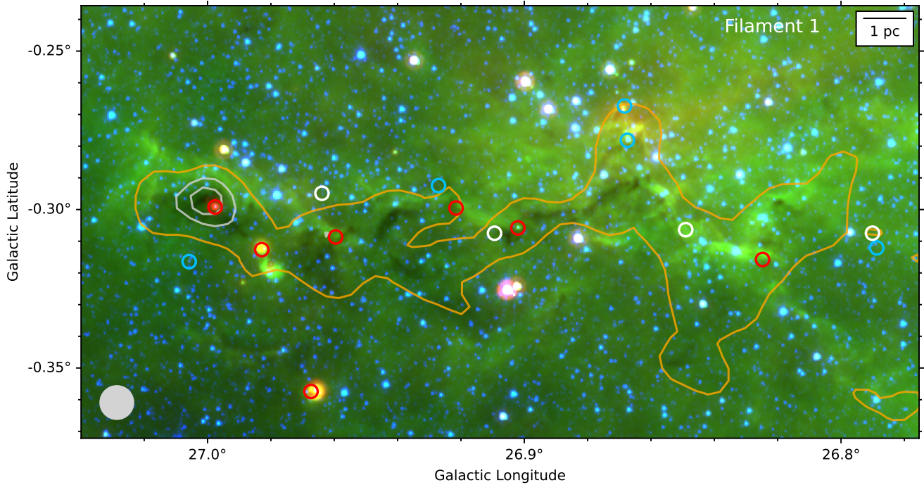
Figure 28. Spitzer red (24 \mu\text{m} ), green (8.0 \mu\text{m} ), and blue (3.6 \mu\text{m} ) composite image for Filament 1. The color levels were chosen to highlight infrared-dark features. Class I and Flat Spectrum (red), Class II (blue), and Class III (white) YSOs from the literature are identified with circles. The three contours trace Herschel -derived N_{\text{H}_2} column densities of 0.5, 1.0, and 1.5 \times 10^{22} \text{ cm}^{-2} , with the lowest level identified in orange for clarity. The Herschel beam is given by the gray circle at the bottom left.
