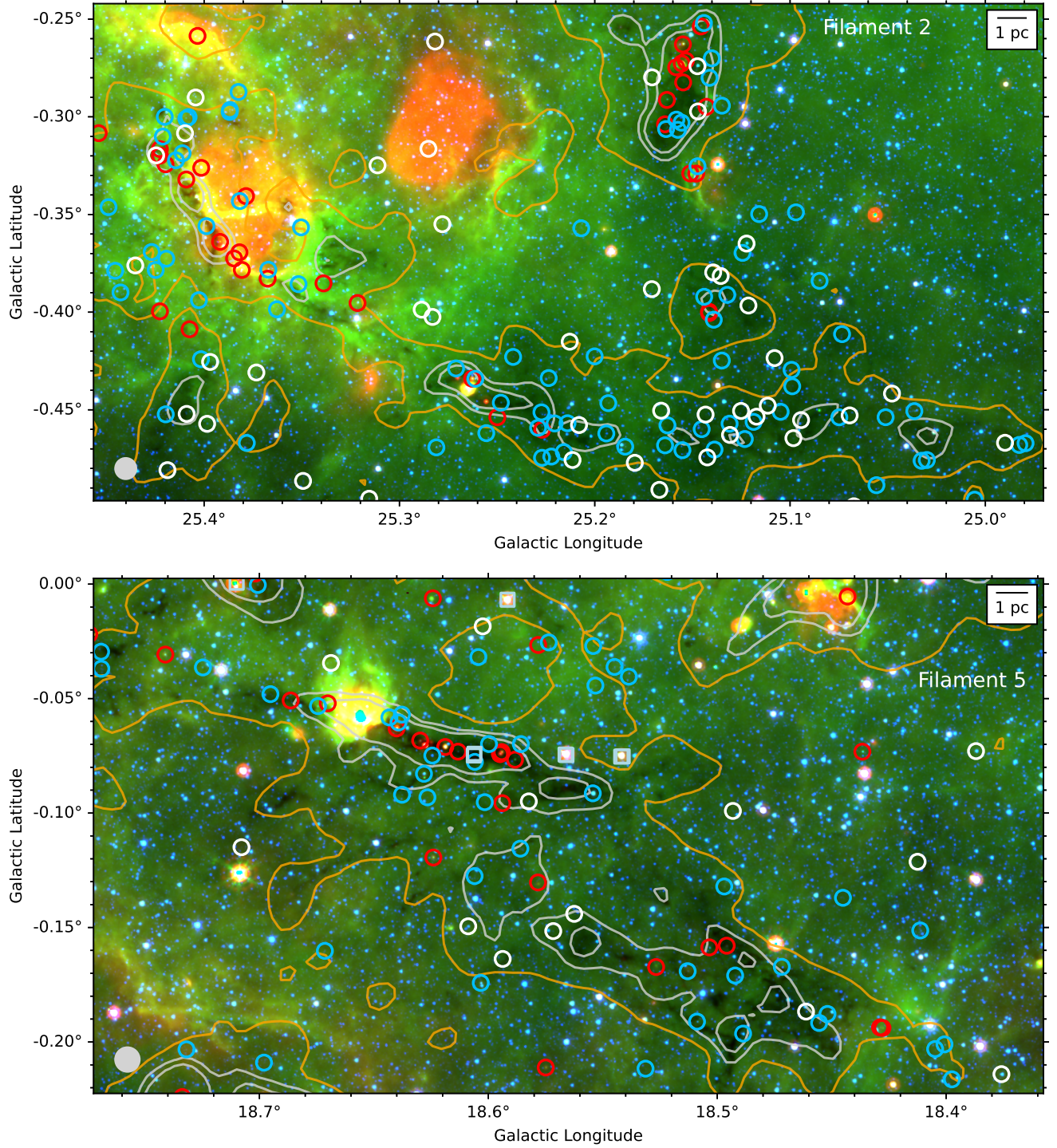
Figure 29. Spitzer red ( 24\ \mu\text{m} ), green ( 8.0\ \mu\text{m} ), and blue ( 3.6\ \mu\text{m} ) composite image for Filament 2 (top) and Filament 5 (bottom). The color levels were chosen to highlight infrared-dark features. Class I (green), Flat Spectrum (violet), Class II (blue), and Class III (red) YSOs from the literature are identified with star symbols. Masers are identified with squares when available. The three contours trace Herschel -derived N_{H_2} column densities of 0.5 , 1.0 , and 1.5 \times 10^{22}\ \text{cm}^{-2} , with the lowest level identified in orange for clarity. The Herschel beam is given by the gray circle at the bottom left.
