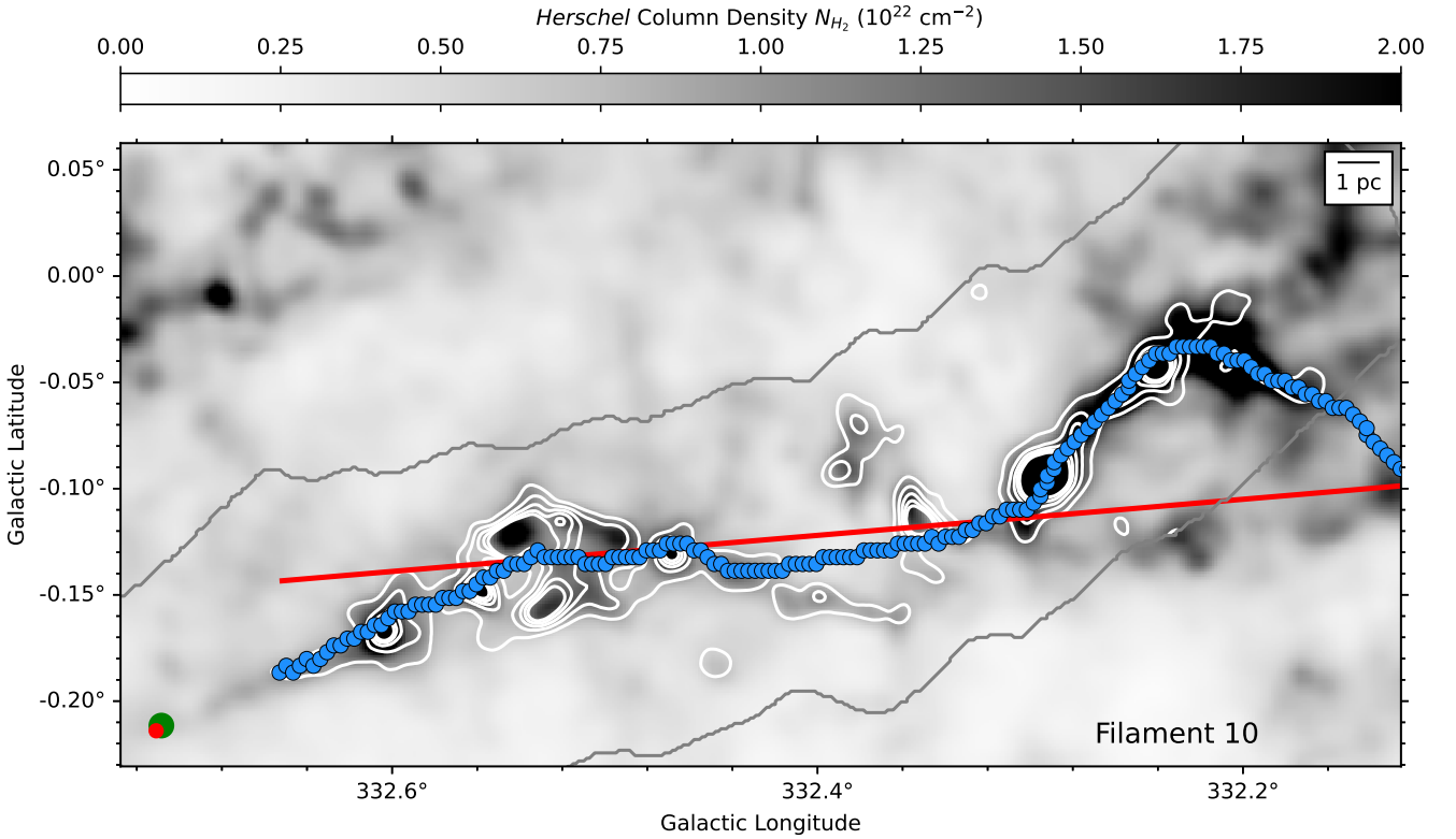
Figure 27. Filament orientation for Filament 10. The blue circles show the result the FILFINDER algorithm for the spine of the filament. The red line is the linear regression used to calculate the filament orientation \phi_F .
