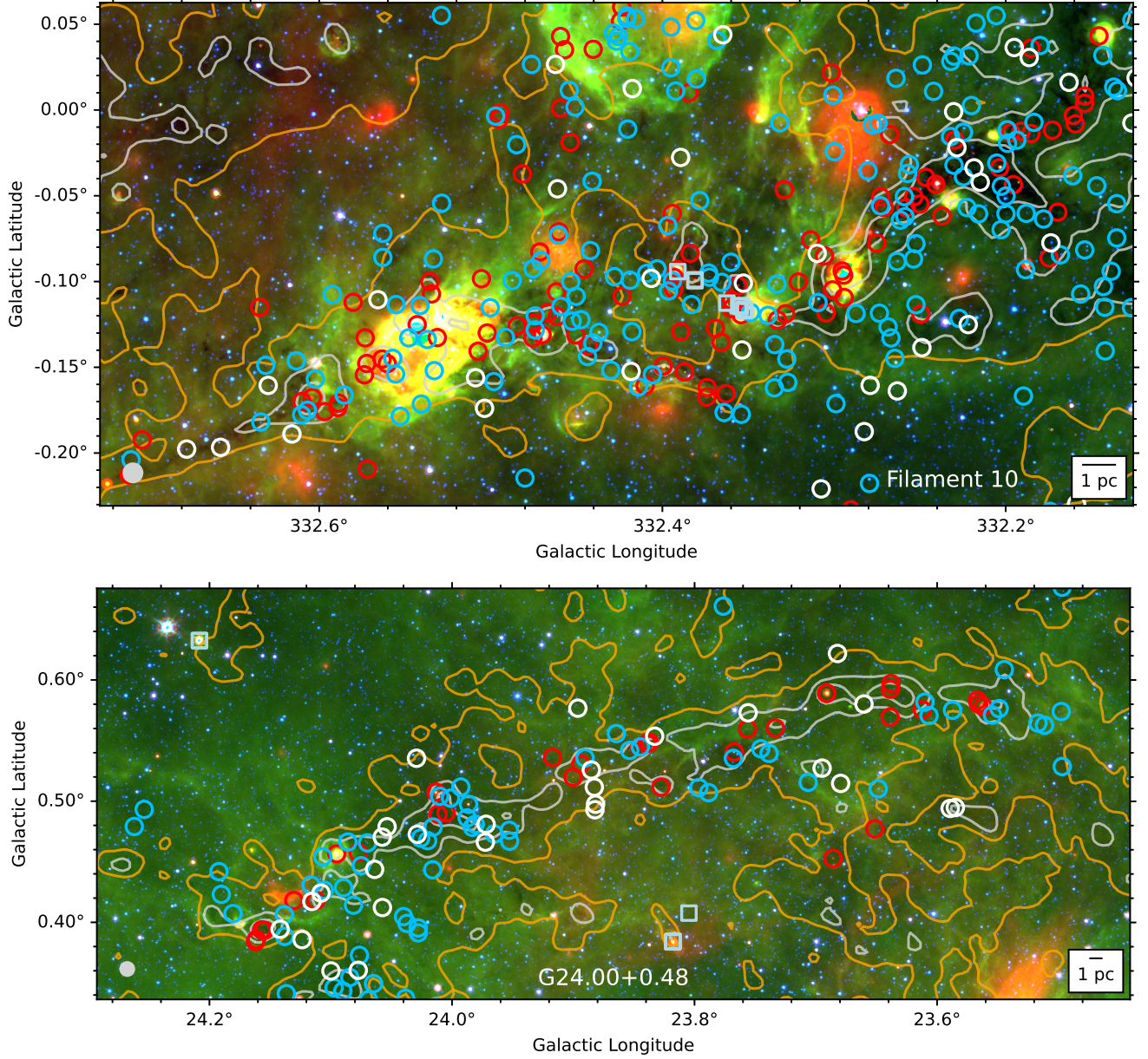
Figure 31. Spitzer red (24 \mu\text{m} ), green (8.0 \mu\text{m} ), and blue (3.6 \mu\text{m} ) composite image for Filament 10 (top) and G24 (bottom). The color levels were chosen to highlight infrared-dark features. Class I (green), Flat Spectrum (violet), Class II (blue), and Class III (red) YSOs from the literature are identified with star symbols. Masars are identified with squares when available. The three contours trace Herschel -derived N_{\text{H}_2} column densities of 0.5, 1.0, and 2.0 \times 10^{22} \text{ cm}^{-2} , with the lowest level identified in orange for clarity. The Herschel beam is given by the gray circle at the bottom left.
