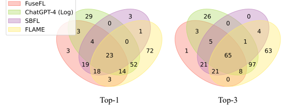
Fig. 5. Distribution of localized faults on PADEFECTS CT .
