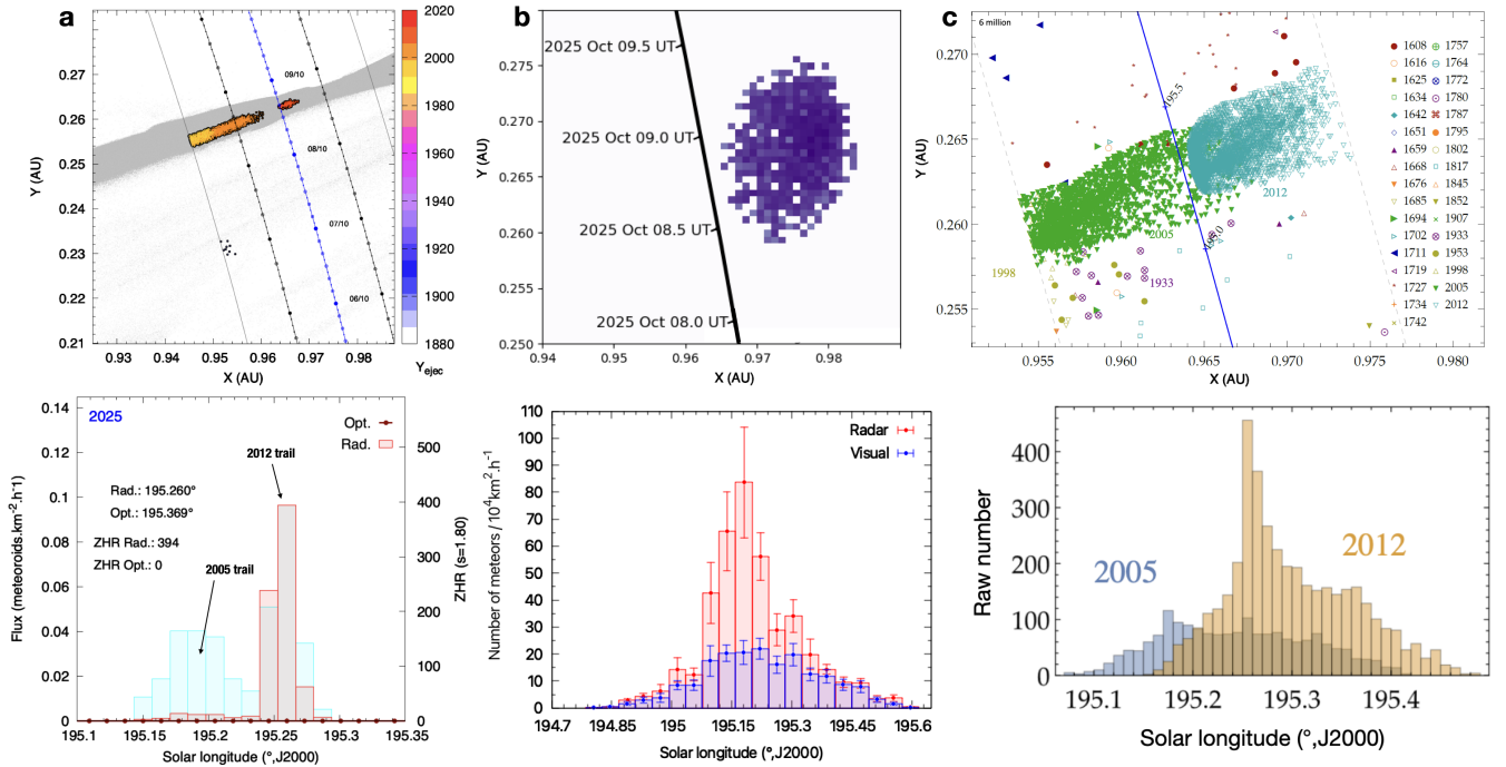
Figure 2. Simulated nodal-crossing locations of Draconid particles (top) and activity profile of the predicted 2025 outburst (bottom), using the NIMS (a), Sisyphus (b), and MSFC (c) models. Only particles crossing the ecliptic plane within the selection criteria ( \Delta X , \Delta T ) from Earth's position are shown in color. Particles released by comet 21P in 2005 and 2012 are shown separately in NIMS and MSFC simulated profiles.
