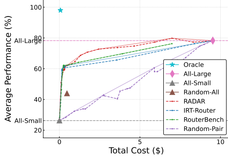
(a) GPQA-Diamond
