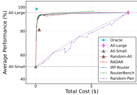
(g) MATH-500
