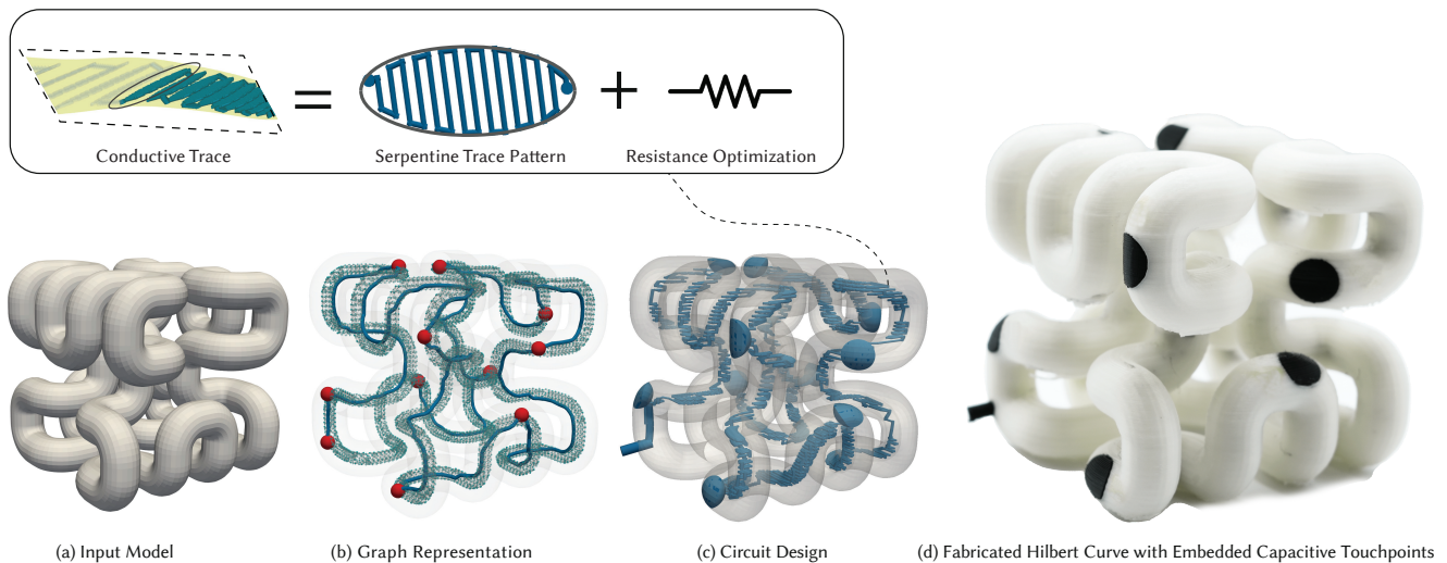
Figure 1: High-level overview of our computational design pipeline: (a) Our pipeline begins with an input model and the user selects different areas on the model's surface to turn into touchpoints; (b) computes a graph-based path to serially connect the touchpoints; (c) generates an internal circuit design to embed capacitive sensors inside the object; and (d) fabricates the object and internal circuit using multi-material 3D printing to be used as a sensing interface with only 1 or 2 wire connections.
