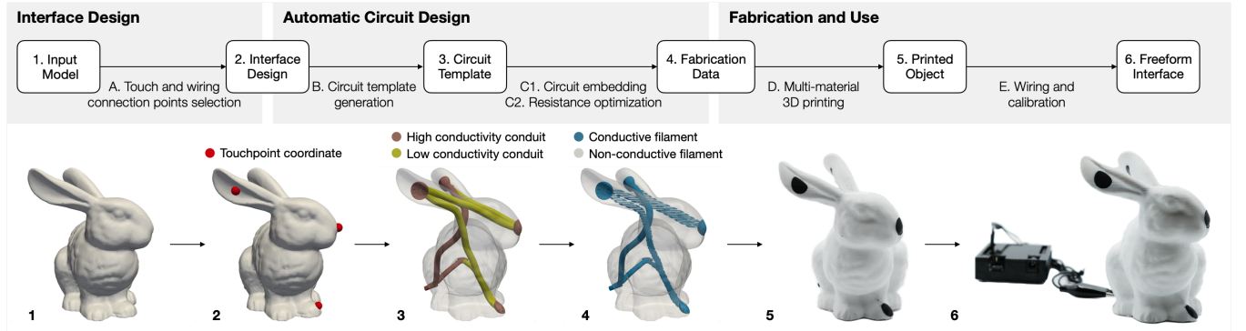
Figure 3: A computational design pipeline to create a freeform interface with embedded capacitive touchpoints. Rounded rectangles represent output data or physical objects. Arrows represent different processes. Each image at the bottom is the corresponding output data (i.e., rounded rectangles) from the computational pipeline.
