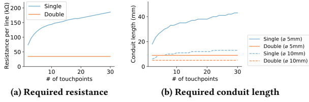
Figure 10: Fabrication scalability evaluation of the single- and double-wire connections with different numbers of touchpoints. In (b), we assume that a conduit has a fixed diameter of 5mm (our pipeline’s default) or 10mm.
