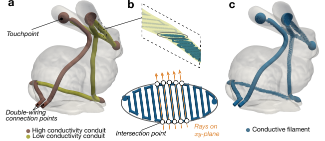
Figure 5: Automatic circuit design. (a) Our automatic circuit design first generates a circuit template, which outlines how we will embed the touchpoints and conductive traces inside a freeform interface. (b) During circuit embedding, serpentine trace patterns are generated inside low conductivity conduits by using a space-filling algorithm. (c) The output is fabrication data (STL files), which will be used for multi-material printing.
