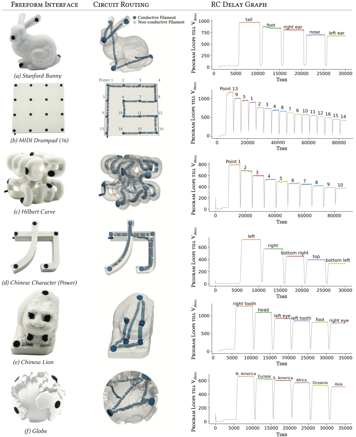
Figure 9: Examples of freeform interfaces with a single-wire connection designed with our computational design pipeline. Each row shows the 3D printed object, its internal circuit design, and its corresponding RC delay graph. The RC delay graph is made by touching each touchpoint one after another. The x -axis corresponds to the time elapsed since using the freeform interface. The y -axis corresponds to the number of program loops that elapsed until reaching the microcontroller's voltage threshold. The RC delay graph is colored based on each touchpoint's unique RC delay (e.g., gray: no touch, orange: first touchpoint).
