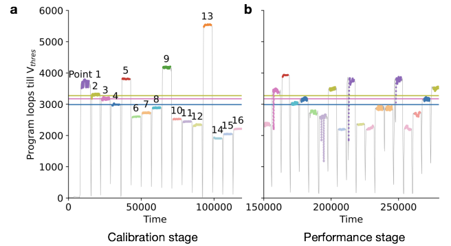
Figure 12: The RC delay graphs from P5's calibration and performance data for PAD_16 with the double-wire connection. Each graph is colored based on the target touchpoint. The colored horizontal lines highlight the mean RC delays measured during the calibration stage (yellow: Point 2, pink: Point 3, blue: Point 4). In (b), we observe that the RC delay of each target node is shifted upwards. For example, a horizontal line shows how Point 4 (blue) in the performance data corresponds to Point 3 (pink), resulting in a misrecognition.
