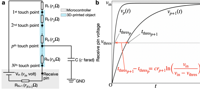
Figure 7: Analysis of a double-wire connection. (a) shows the circuit schematic for the double-wire connection, where the p th touchpoint is selected. (b) compares the voltage changes and time delays induced when p th and (p+1) th touchpoints are touched.
