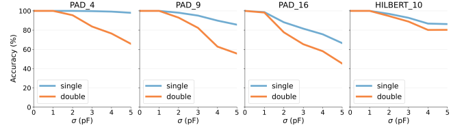
Figure 13: Results from the capacitance perturbation simulation for the freeform interfaces. \sigma represents the strength of the perturbation (specifically, capacitance values are sampled from a Gaussian distribution with \mu = 100\text{pF} and \sigma ). The single-wire connection is more robust to the capacitance shift than the double-wire connection.
