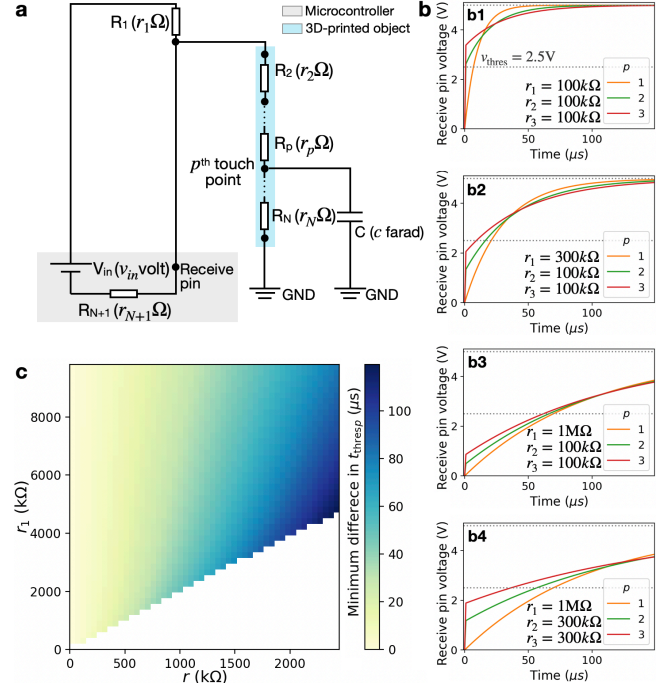
Figure 8: Analysis of a single-wire connection. (a) shows the circuit schematic for the single-wire connection where the p th touchpoint is selected. (b) compares the voltage changes across different variations of three resistance values ( r_1, r_2, r_3 ). (c) shows the minimum differences among t_{thres_1}, t_{thres_2}, t_{thres_3} for the different variations of r_1 and r (note: here r_2=r_3=r ). A white grid cell indicates a violation of the hard constraint of r_1 . For (b) and (c), we assume a case using the Arduino UNO R4 (i.e., v_{in} = 5 V, v_{thres} = 2.5 V) and c = 100 pF.
