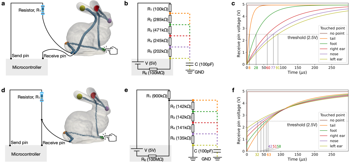
Figure 2: Capacitive sensing for the Stanford Bunny: (a) overall schematic on how the five touchpoints are connected via conductive traces (colored blue) and connected in series to a microcontroller’s circuit using two wires; (b) the circuit diagram corresponding to (a) with the representative resistance and capacitance measurements. Each colored dashed wire corresponds to a case when a point is touched (e.g., orange: tail, green: foot); and (c) the voltage change measured at the microcontroller’s receive pin when a point is touched. (d–f) correspond to (a–c) but the Stanford Bunny is connected in parallel to a microcontroller’s circuit using one wire.
