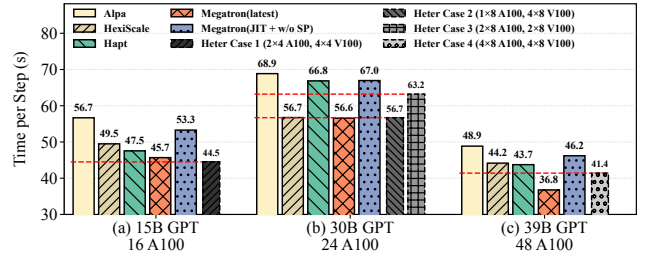
Figure 9. Comparison of end-to-end training latency across homogeneous and heterogeneous GPU clusters.
