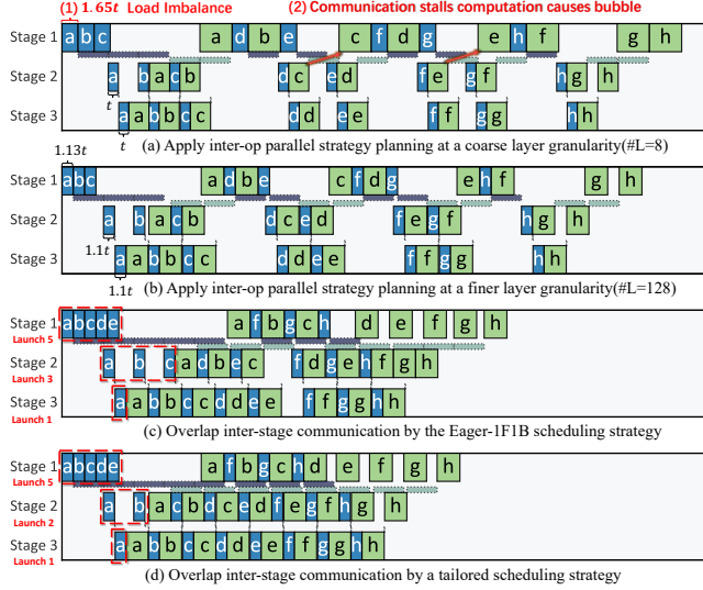
Figure 3. Pipeline timeline of case studies.
