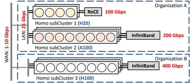
Figure 1. Example heterogeneous cluster composed of multiple homogeneous subclusters, with fast interconnects within subclusters but slower interconnects across them.
