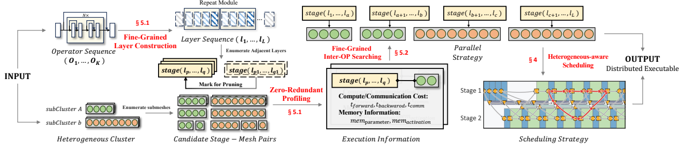
Figure 4. Overview of HAPT workflow.
