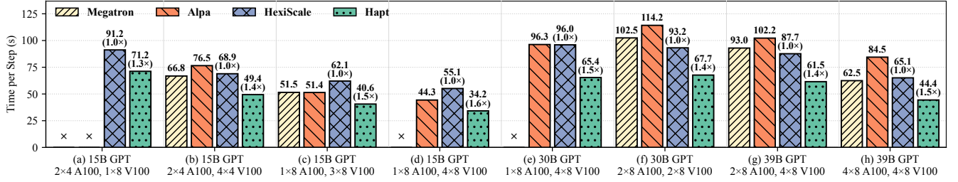
Figure 7. End-to-end training latency of Hapt compared with baselines under different heterogeneous configurations.
