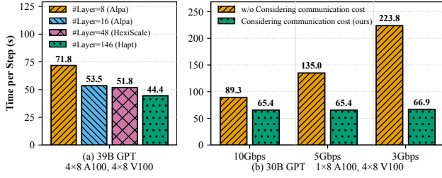
Figure 11. (a) Effect of fine layer granularity, (b) Effect of joint optimization of planning and scheduling.
