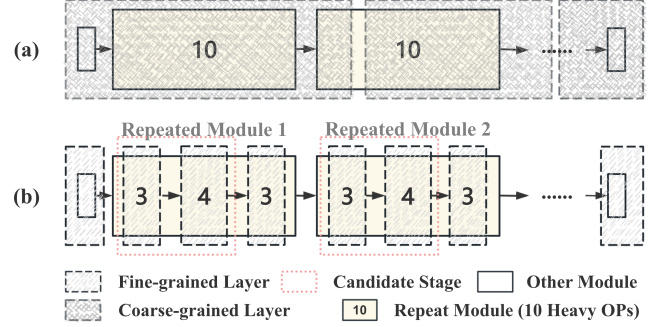
Figure 6. (a) Behaviour of layer construction in Alpha. (b) Behaviour of layer construction in Zero-Redundant Profiler.
