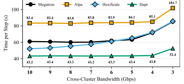
Figure 10. End-to-end training latency of different systems under varying cross-cluster bandwidths (3–10 Gbps).
