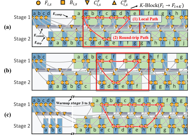
Figure 5. DAG representation of the pipeline execution. (a) Two-stage homogeneous case where the local path dominates K -block latency. (b) Two-stage homogeneous case where the round-trip path dominates K -block latency. (c) S -stage homogeneous case, reduced to an equivalent two-stage subgraph by pruning nodes & edges unrelated to stages 1–2.
