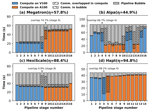
Figure 8. Stage-wise breakdown of computation, communication, and idle bubbles within one iteration for the configuration in Figure 7(h). For each framework, we annotate the communication-latency overlap ratio at the stage located on the subcluster boundary.
