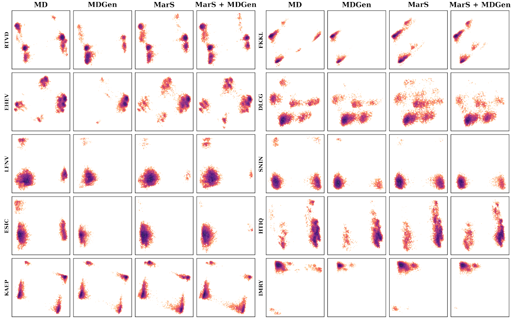
Figure 6: TICA plot for 10 random peptides in the test set, comparing MD ground-truth, MDGen, MARS (ours) and MARS + MDGen (ours). Our frameworks explore modes that are otherwise entirely ignored by MDGen.
