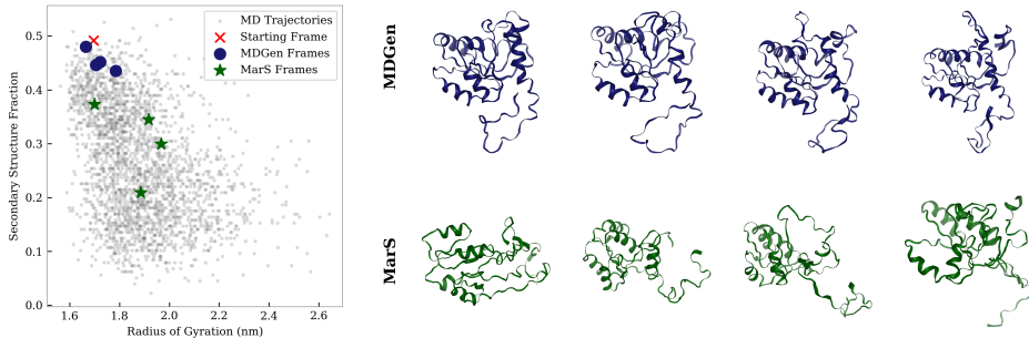
Figure 5: First 4 samples generated by MDGen and MARS-FM for the domain 2ynmD03 in the test set. As MARS-FM interpolates among states independently of temporal dynamics, it can explore the energy landscape more efficiently. In fact, the secondary structure content varies significantly among these 4 samples (note that there is no ordering as they are generated in parallel). Conversely, MDGen samples all belong to the same energy minimum which reduced sampling efficiency and exploration.
