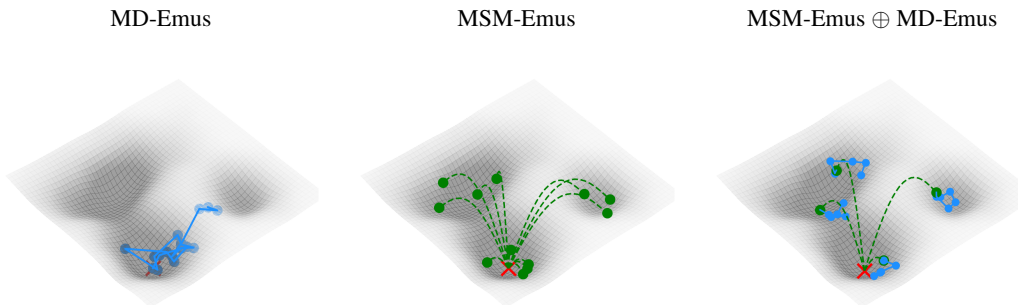
Figure 1: Comparison between existing approaches (MD-Emus) and our proposed novel class (MSM-Emus). MD-Emus learn transitions within a state (i.e. energy minima) well but could fail to generate transitions across different states (minima) since they are constrained by the data imbalance intrinsic to MD. Conversely, our framework learns to sample from the distribution induced by a Markov State Model (MSM). This modeling shift means that generative models are decoupled from temporal dynamics and can better learn to sample inter-state transitions. During sampling, MSM-Emus can generate conformations in parallel or be combined with existing MD-Emus to capture both large conformational changes as well as local dynamics within states.
