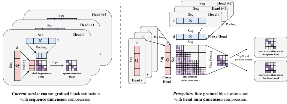
Figure 3: Illustration of ProxyAttn. By compressing the head dimension, ProxyAttn can obtain token-level importance scores, leading to more accurate block importance estimation. A proxy head is able to obtain diverse masks by leveraging the online budget estimations from different heads.
