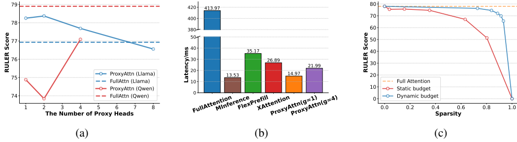
Figure 5: Experimental analysis of proposed method. (a) The performance of different numbers of proxy attention heads across various models. (b) Latency for estimating block importance with 128K inputs using different methods. The latency of all methods is less than 10% of the Full Attention. (c) Performance degradation with increasing sparsity rate for different budget allocation methods.
