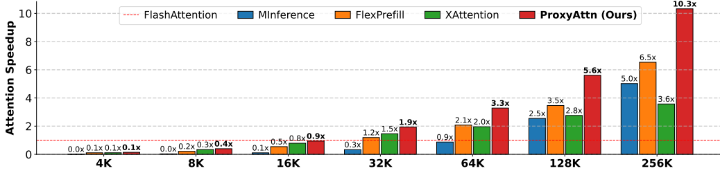
Figure 4: Kernel-level speedup of existing sparse attention methods with varying input lengths.
