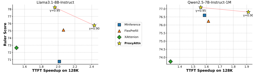
Figure 1: Performance and speedup results of different sparse attention methods on RULER.
