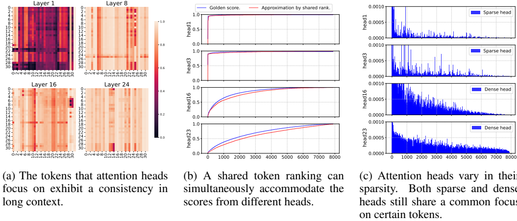
Figure 2: Observational study on Llama3.1-8B-Instruct using 8K-token data from the Needle in a Haystack (NIAH) Single-1 task of the RULER (Hsieh et al., 2024) dataset.
