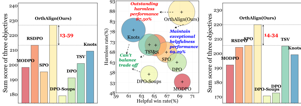
Figure 1: (Left) Average three-objective performance on Llama3-SFT (Dong et al., 2024); (Middle) Two-objective average performance on all configurations; (Right) Average three-objective performance on Mistral-SFT (Tunstall et al., 2023).
