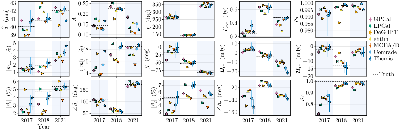
Fig. 5. Comparison of extracted parameters for the blinded synthetic data test. All methods are blurred to match the ground truth GRMHD, blurred to 20\mu\text{as} before the parameters are estimated. The markers show the results for each method. For the two Bayesian methods, Comrade and Themis, the markers denote the median, and the error bars the 95% credible interval. Since the synthetic data only consider a single frequency, the non-Bayesian methods only produce a single image. The dashed black line shows the ground truth, estimated from the true on-sky image blurred with a 20\mu\text{as} Gaussian beam.
