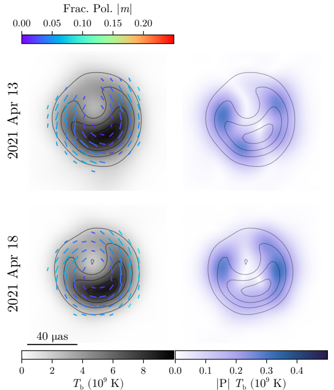
Fig. A.4. Fiducial images from April 13, 2021, and April 18, 2021. The April 13 image is constructed in the same manner as Fig. 6.
