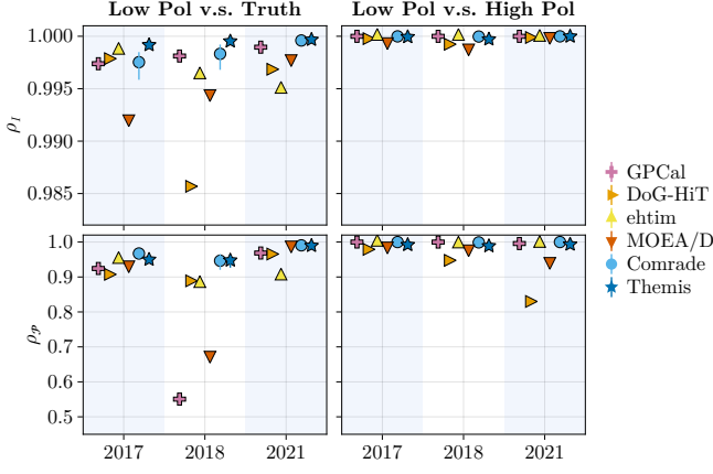
Fig. D.3. Cross-correlation between the low polarized and high polarized extended jet geometric tests. The ring model for the two tests is identical, meaning that the cross-correlation in the core region would be equal to unity for perfect reconstructions. Left column: Total intensity (top row) and linear polarization cross-correlation (bottom row) between the low-polarized jet reconstructions. Right column: Same quantities but with the cross-correlation computed between the low and high polarized jet reconstructions.
