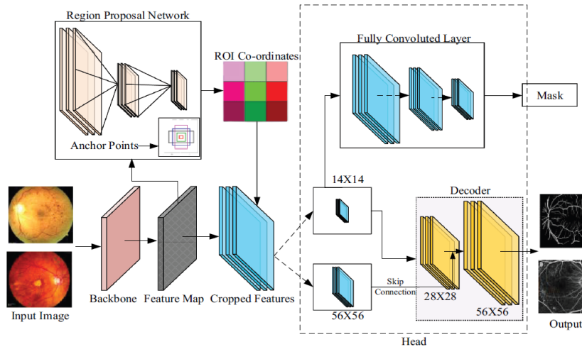
Figure 3. Process of segmentation of blood vessels using improved mask R-CNN [28]
