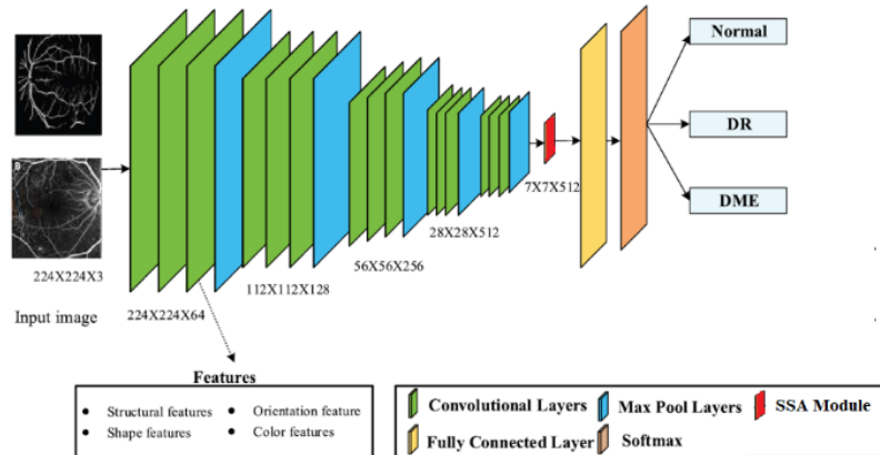
Figure 4. Process of extraction of features and classification using SSA-VGG-16 [28]
