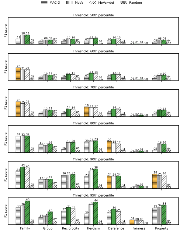
Figure X: F1 score using different thresholds
