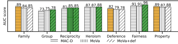
Figure IX: AUC scores across 7 moral dimensions on the MAC dataset.
