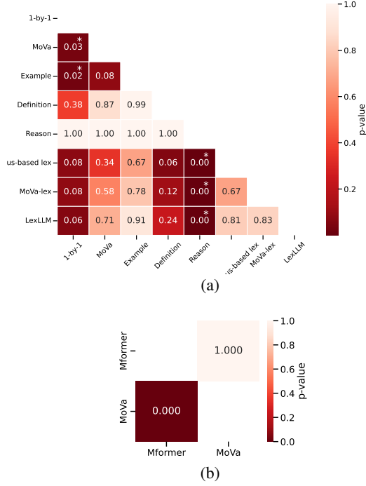
Figure VIII: Wilcoxon signed-rank test results. (a) Wilcoxon signed-rank test for prompting strategies using in-domain evaluation. (b) Wilcoxon signed-rank test results for MoVa vs Mformer using out-domain evaluation. Significant results (p-value < 0.05) are marked with a star (*), (p-value < 0.01) marked with two stars (**) and (p-value < 0.001) marked with three stars (***).
