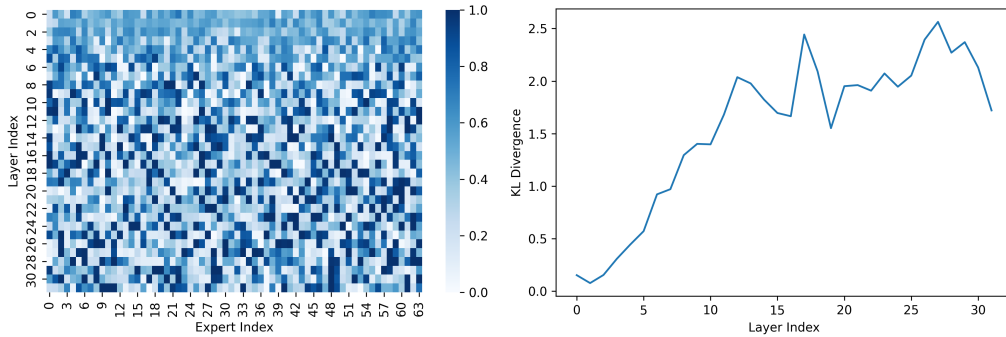
Figure 8: Left: Heatmap of \frac{v_{ij} t_{ij}}{\sum_j v_{ij} + \sum_j t_{ij}} , where v_{ij} and t_{ij} denote the image-token and text-token activation counts, respectively, for the j -th expert in the i -th layer. The darker an expert appears, the more specialized it is to image tokens. Right: KL divergence between \{\frac{v_{ik}}{\sum_j v_{ij}}\}_{k=0}^{64} and \{\frac{t_{ik}}{\sum_j t_{ij}}\}_{k=0}^{64} for all experts of each layer. As the layer goes deeper, the KL divergence increases and the expert activation distributions become more dispersed across modalities.
