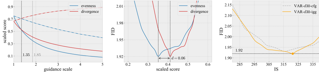
Figure 4: Analysing the relationships between various metric scores attained by VAR-d30-IGG. From left to right: effect of changing guidance scales on reported evenness and divergence scores, where dashed and solid lines depict raw and scaled scores respectively; correspondence between FID and scaled evenness and divergence scores; and FID-IS trade-off curve.
