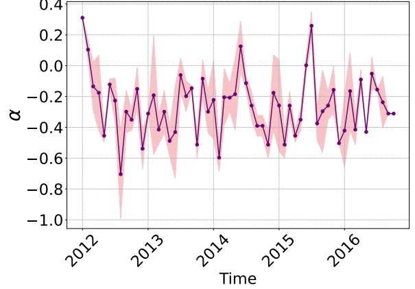
Figure 5: Why extrapolation does not work? The optimal extrapolation factor \alpha fluctuates with time and is often less than one or even negative. This indicates that sometimes interpolation is preferable over extrapolation for temporal generalization.
