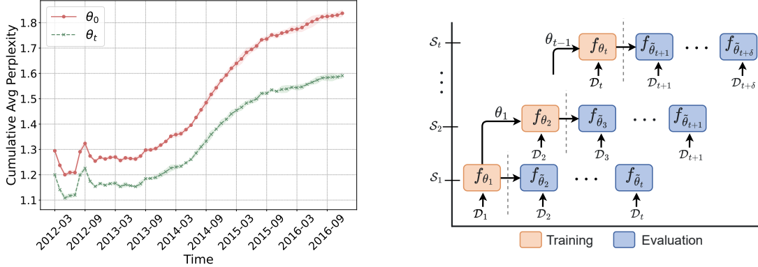
Figure 1: (Left) Performance degrades over time. The widening performance gap between a stale model trained once in January 2012 (red) and a monthly updated model (green) illustrates the decay in performance over time. The evaluation was conducted using data from March 2012 onward. (Right) Temporal generalization framework. Across sequential learning stages ( S_t on the y-axis), a model f_{\theta_t} is trained on data \mathcal{D}_t (orange) initialized with \theta_{t-1} from the previous stage. This generates a sequence of historical parameters. This sequence is used to estimate future parameters \theta_{t+\delta} , which are used to evaluate future data (blue) \mathcal{D}_{t+\delta} for \delta > 0 (x-axis).
