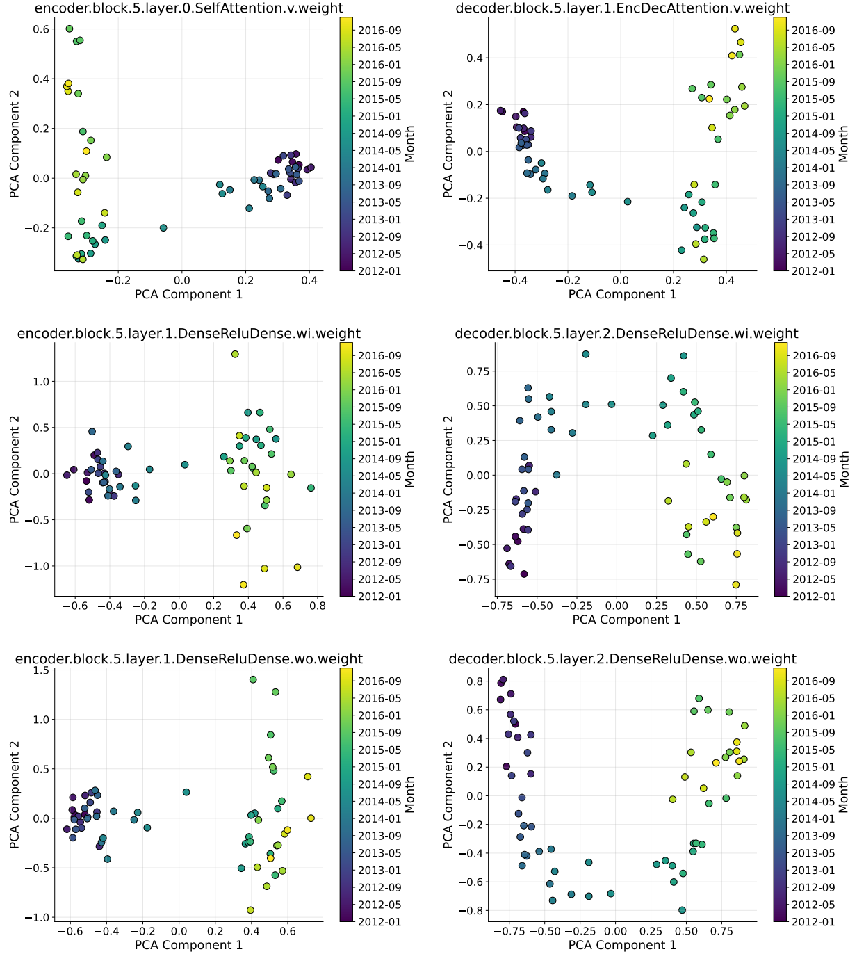
Figure 15: Parameter trajectories from independent finetuning. PCA of T5-small weights during news summarization, where each timestamp model is trained independently from a pre-trained checkpoint. The lack of smoothness across time steps indicates inconsistent parameter evolution and highlights the challenges of extrapolation in the absence of continual learning.
