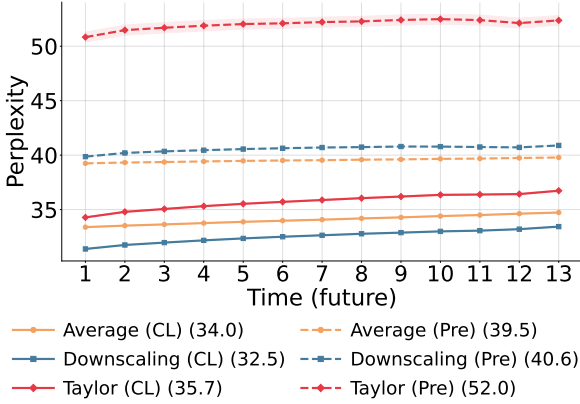
Figure 6: For language modelling, CL (solid lines) improves average perplexity compared to pre-trained model (dashed lines).
