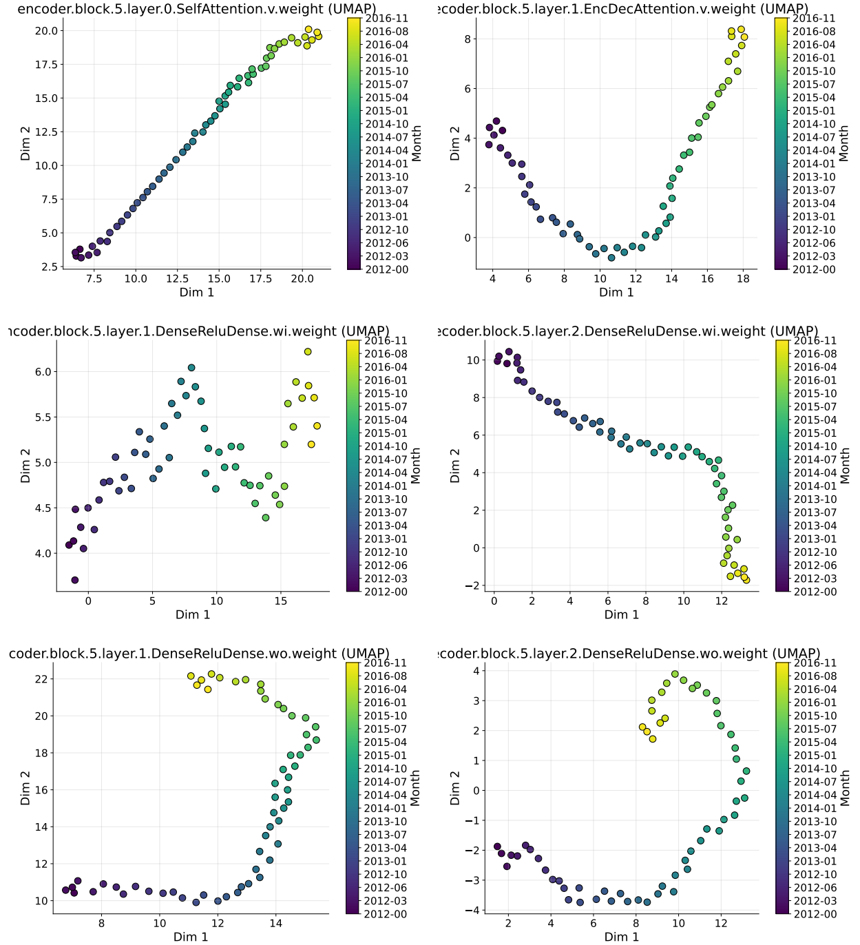
Figure 19: UMAP under continual learning. UMAP of T5-small weights during language modeling with continual learning.
