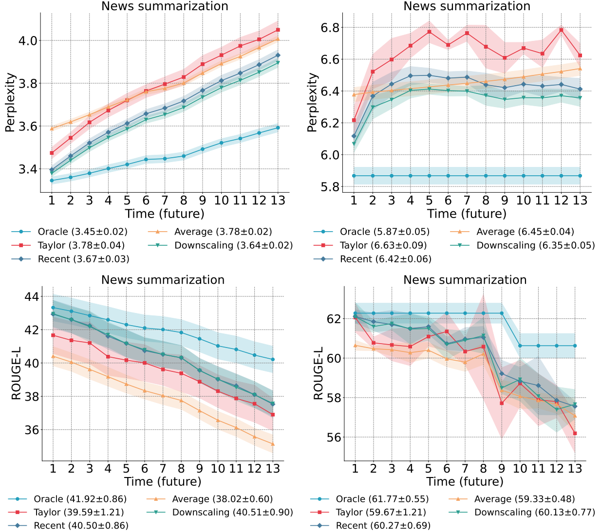
Figure 11: Perplexity and ROUGE-L comparison for T5-large model. We contrast average-case performance (left panels) with worst-case performance (right panels) over future time steps (x-axis). Effective summarization is marked by lower Perplexity scores and higher ROUGE-L scores (y-axis). Downscaling is the only method that does not consistently lead to performance decay across both evaluation metrics compared to the recent model.
