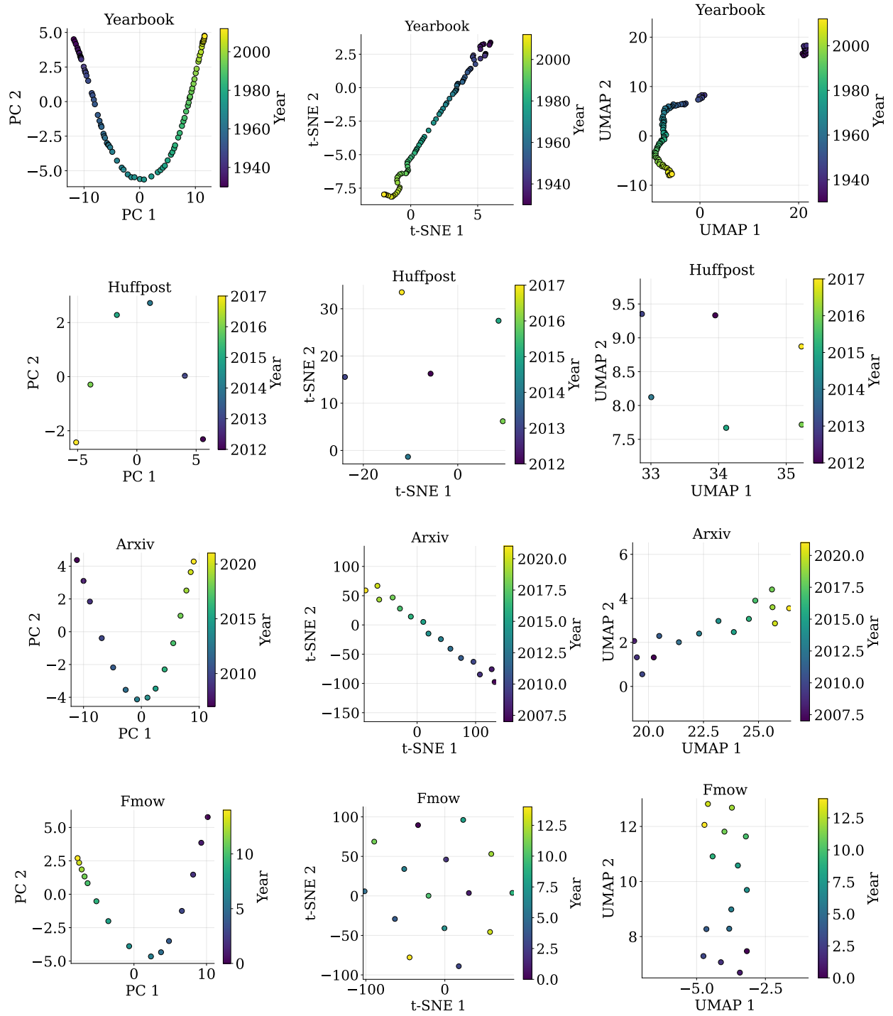
Figure 13: Dimensionality reduction of model parameters over time for WILDS-Time datasets. Each scatter plot shows a 2D projection of model checkpoints using PCA, TSNE and UMAP dimensionality reduction techniques.
