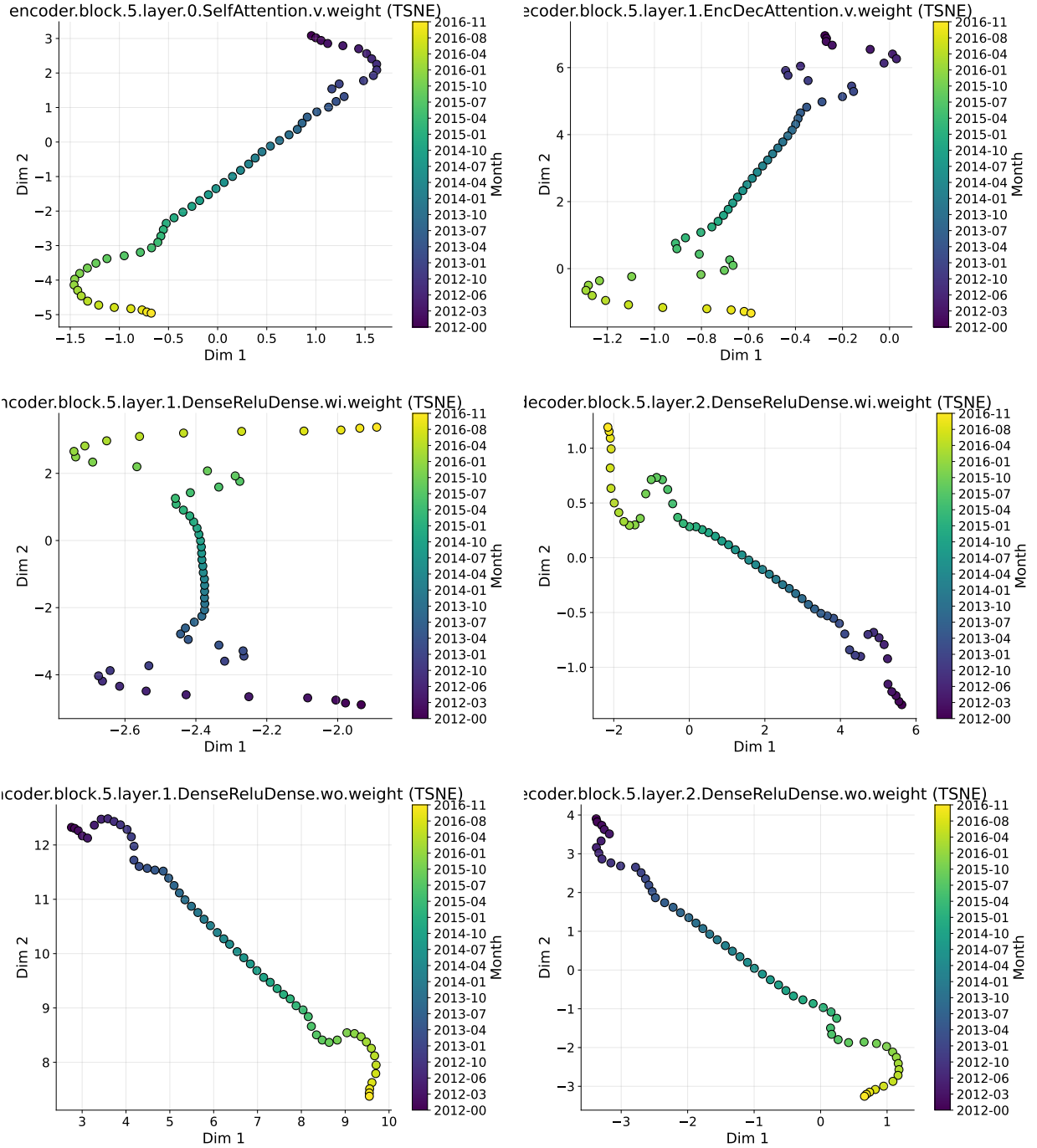
Figure 17: TSNE under continual learning. TSNE of T5-small weights during language modeling with continual learning.
