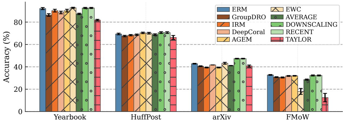
Figure 3: Comparison of ERM (trained on union of data up to time t ) with DG (GroupDRO [Sagawa et al., 2020], IRM [Arjovsky et al., 2019], DeepCoral [Sun and Saenko, 2016]), CL methods (EWC [Kirkpatrick et al., 2017], AGEM [Chaudhry et al., 2019]), parameter interpolation (Average, Downscaling, Recent), and Taylor extrapolation over \delta future months. No method consistently outperforms others across datasets. The details for the methods are provided in Section E.
