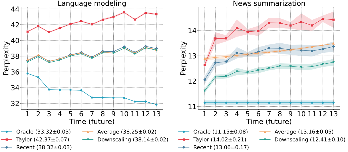
(a) Worse-case Perplexity for T5-small model. The left panel shows results for language modeling and the right panel for news summarization. Each method is evaluated over future time steps (x-axis), with lower Perplexity values (y-axis) indicating better performance. Consistent with the average-case performance, we see that only downscaling does not lead to a drop in performance compared to a recent model.
