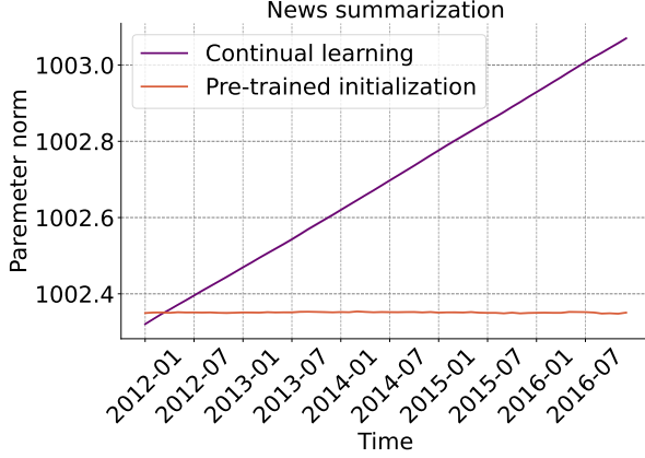
Figure 4: Why downscaling works? The L2 norm of model parameters increases over time under continual learning, while it remains flat for models reinitialized at each step. Downscaling reduces this overconfidence and improves temporal generalization.
