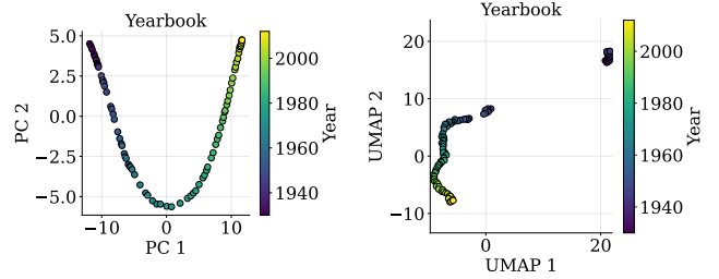
Figure 7: Dimensionality reduction with PCA (left) and UMAP (right) on models trained with yearbook dataset showing the change of parameters with time.
