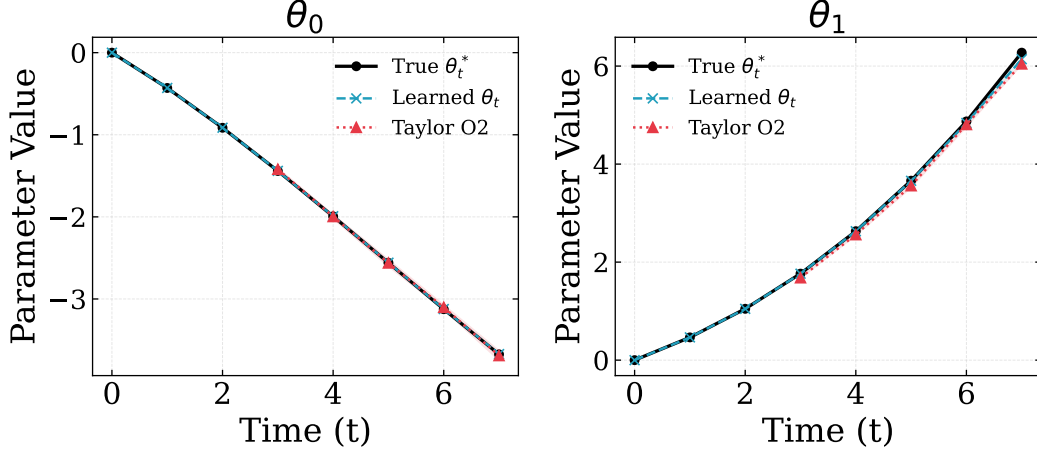
Figure 8: Comparison of true underlying parameters \theta_t^* , learned parameters \theta_t of a linear model and Taylor second-order extrapolated parameters \theta_t . The identical plots for the true parameters and extrapolated parameters illustrate effective parameter estimation.
