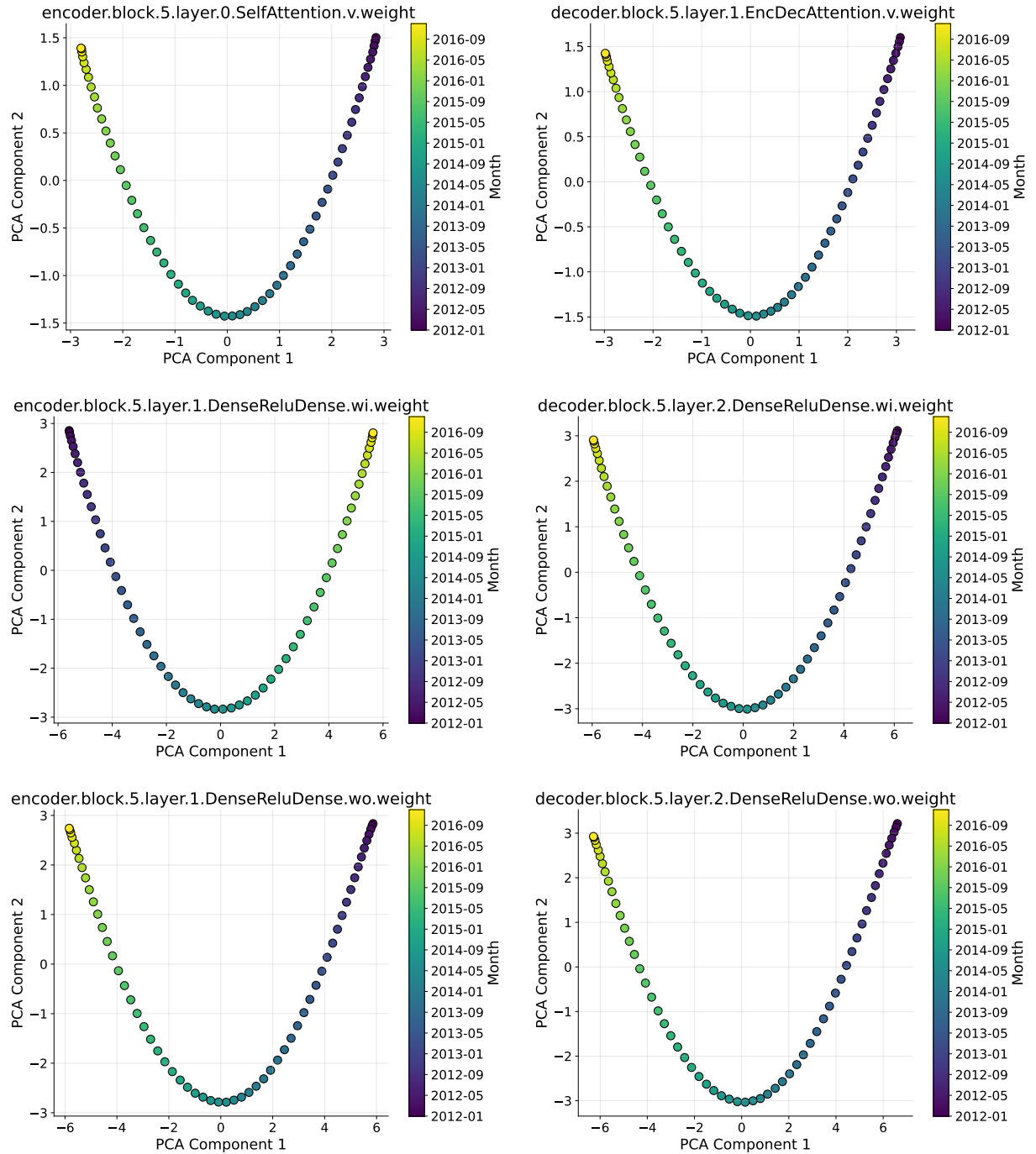
Figure 14: Smooth parameter trajectories under continual learning. PCA of T5-small weights during news summarization with continual learning shows smooth, coherent evolution over time. This contrasts with independently fine-tuned checkpoints (Figure 15), highlighting how continual learning preserves temporal consistency in parameter space and supports forward transfer.
