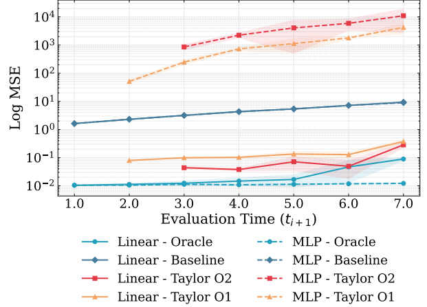
Figure 10: Log MSE Extrapolation Performance: One-step-ahead performance comparison for linear (solid lines) and MLP (dashed lines) models. The linear model with identifiable parameters allows for more effective Taylor extrapolation than MLP, whose parameter non-identifiability impedes performance. The oracle performance of linear and MLP overlaps.
