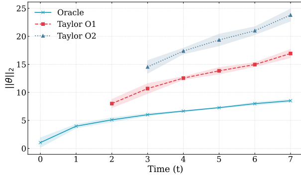
Figure 9: MLP Parameter Norm Evolution: \ell_2 norm comparison of MLP Oracle, and extrapolated parameters using Taylor O1 (first-order) and O2 (second-order) approximations. The divergence in extrapolated norms highlights challenges in extrapolating MLP parameter trajectories across time.
