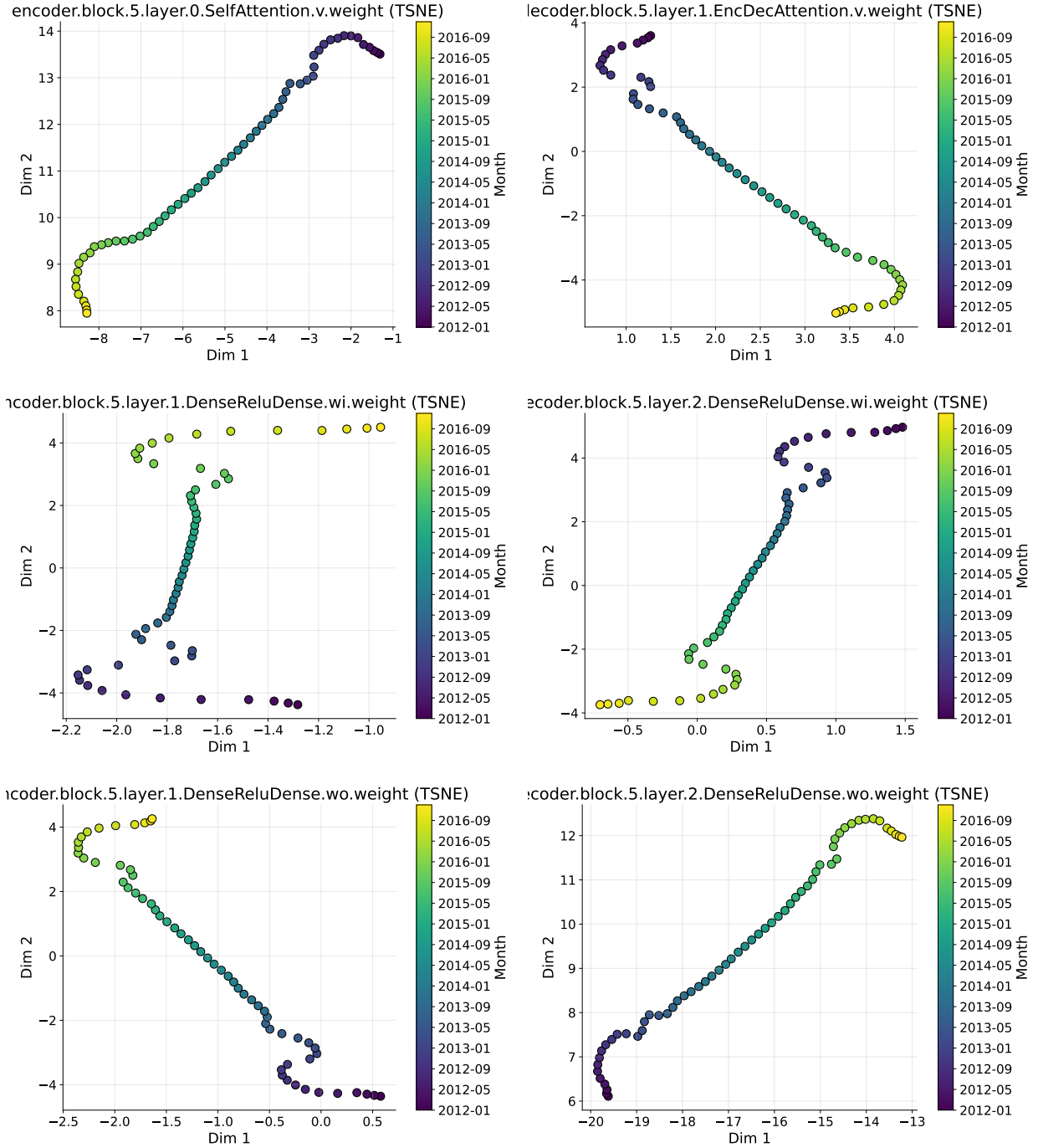
Figure 18: TSNE under continual learning. TSNE of T5-small weights during news summarization with continual learning.
