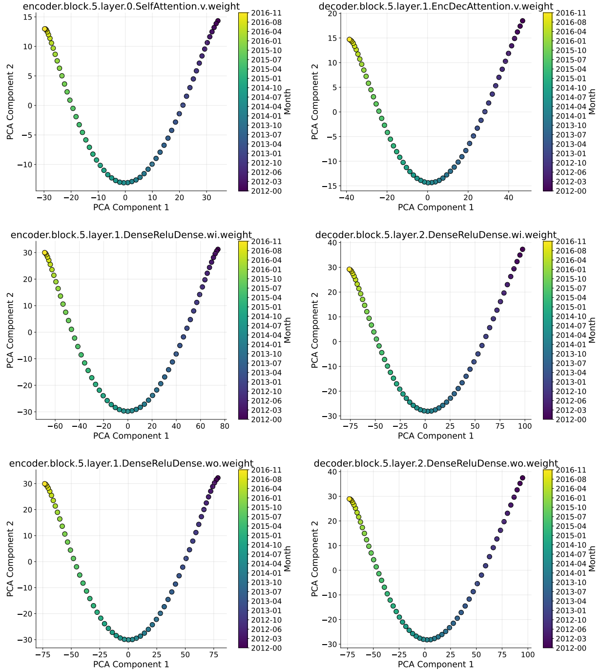
Figure 16: Smooth parameter trajectories under continual learning. PCA of T5-small weights during language modeling with continual learning shows smooth, coherent evolution over time.
