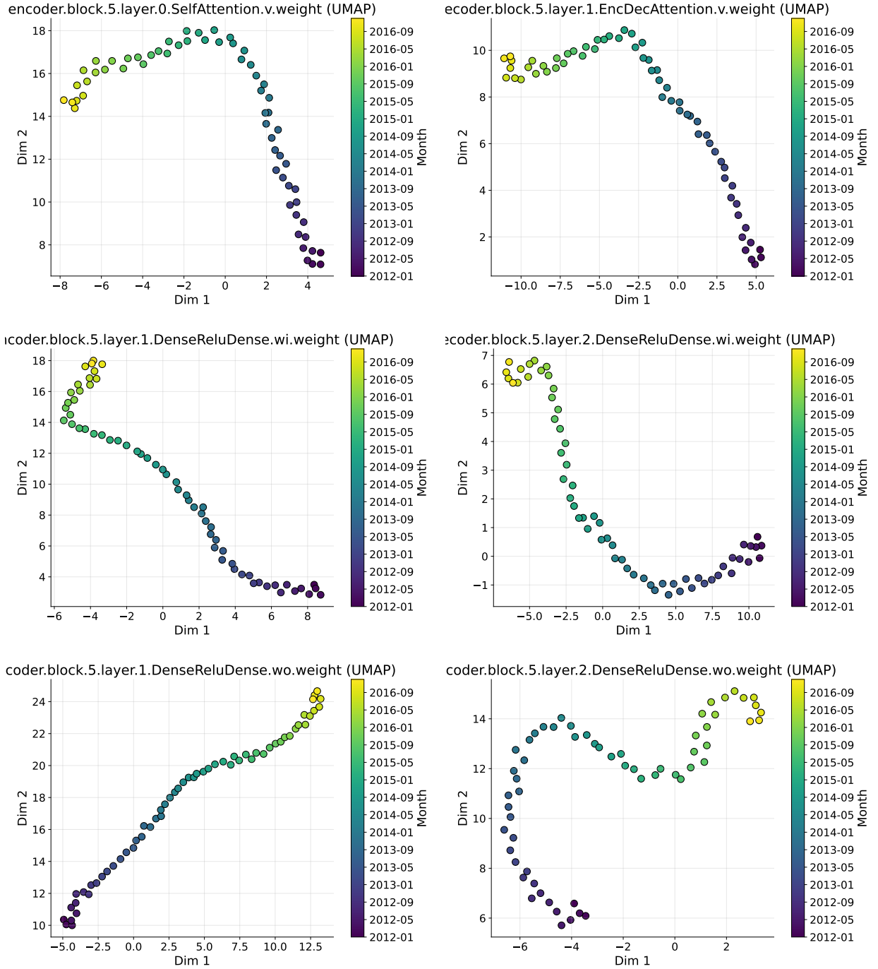
Figure 20: UMAP under continual learning. UMAP of T5-small weights during news summarization with continual learning.
