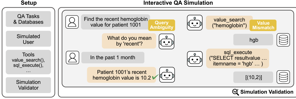
Figure 1: Overview of EHR-ChatQA. Our benchmark places an agent in a simulated environment with an LLM-powered user and tools. The agent must manage the full workflow: clarifying vague user questions, resolving terminology mismatches, generating and executing accurate SQL, and returning the final answer. Each interaction trace is validated for accurate evaluation.
