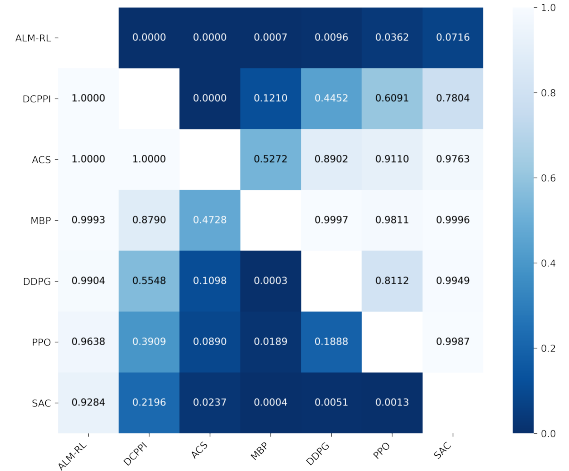
Figure 2: Heatmap of p -values from one-sided Wilcoxon paired tests comparing the terminal reward of each ALM strategy. The terminal reward is calculated as the average reward over the last 500 episodes to reduce the noise that may result from using a single final episode.
