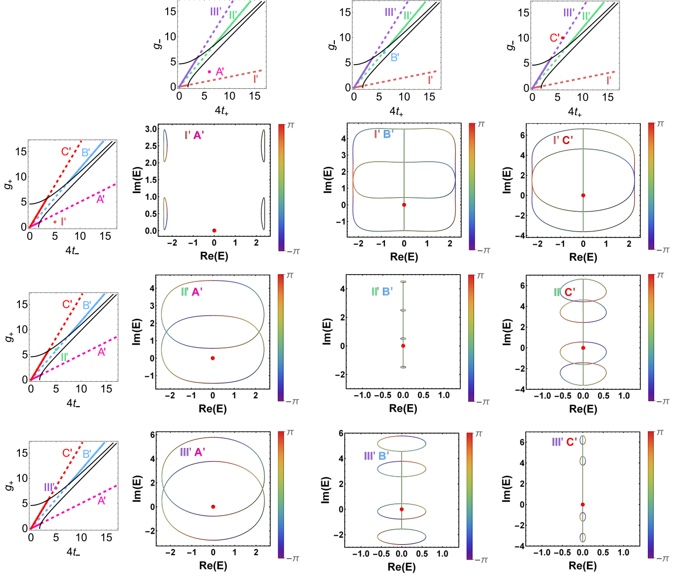
FIG. 19. PBC spectra for H_{+,+} defined in Eq. (19) with the adopted parameter values identical to those in Fig. 11. In each panel, the color map marks the spectral trajectory corresponding to the ka_0 value going from -\pi to \pi , and the red dot marks the origin in the complex energy plane. See Table III for the adopted values of the full parameter sets.
