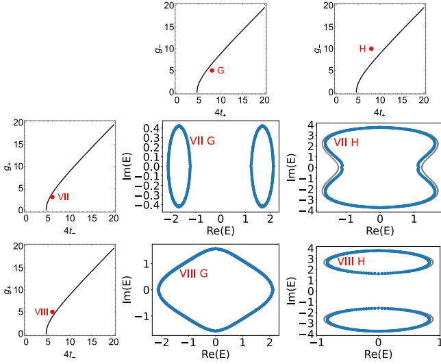
FIG. 14. Parameter diagrams and energy spectra; similar plot as Fig. 5, but with \Gamma'_0 = \Gamma_a = -\Gamma_b = 5 , \Delta_0 = 1 , and \delta h_x = 0.01 . See Table III for the adopted values of the full parameter sets.
