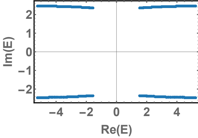
FIG. 18. OBC energy spectra, \pm\sqrt{E_{+, \lambda}^2 + \Delta_0^2} , calculated from Eq. (B13) for the parameter set II A. See Table III for the adopted values of the full parameter set.
