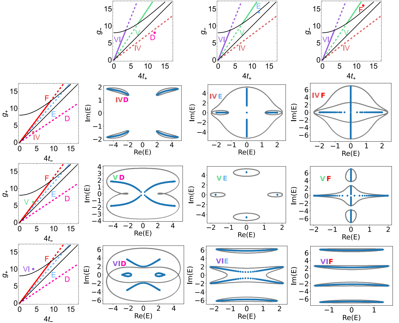
FIG. 17. Similar plots to Fig. 6, except that we have \delta_x = 0 here. See Table III for the adopted values of the full parameter sets.
