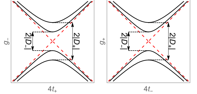
FIG. 2. Gap closing curves for Case (i) in the t_+-g_- (left) and t_-g_+ (right) planes for a general parameter set. The solid curves are derived from Eq. (6) and can be used to deduce phase diagrams. The red dashed lines, |g_\pm| = 4|t_\mp| , correspond to the asymptotic limit of D_\pm = 0 .
