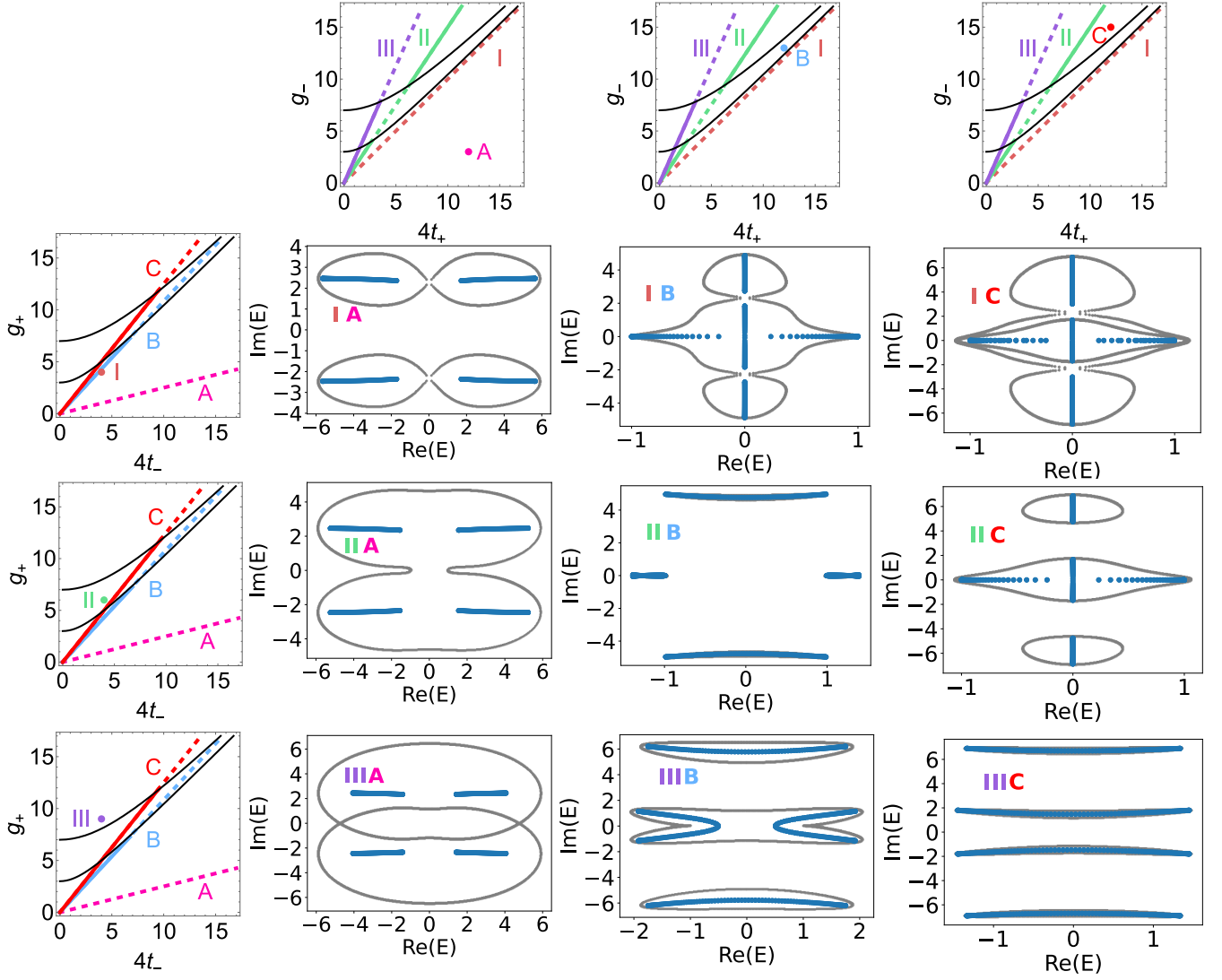
FIG. 16. Similar plots to Fig. 5, except that we have \delta_x = 0 here. See Table III for the adopted values of the full parameter sets.
