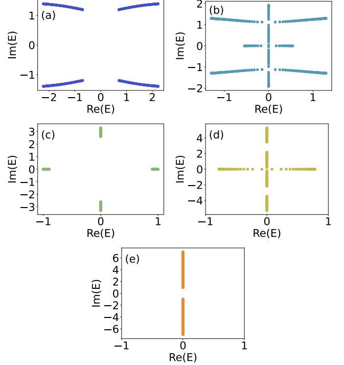
FIG. 13. Energy spectra for Case (iib') with \Gamma_+ = 3 , \Gamma_- = 2 , \Delta_0 = 1 , and C_0 = 0.5 . The spectra are computed at the parameter sets marked by the colored dots in Fig. 9(b), with t_+ = 5/4 and g_- = 2, 4, 6, 9 and 12 . Here, the PBC spectra coincide with the OBC ones. See Table III for the adopted values of the full parameter sets.
