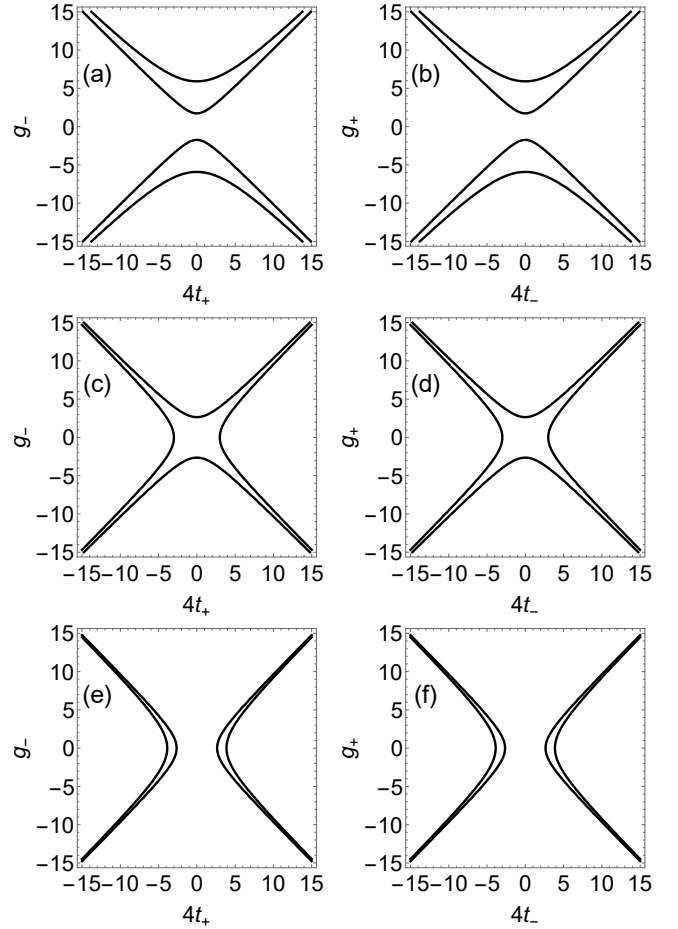
FIG. 8. Gap closing curves in the t_+-g_- (left column) and t_-g_+ (right column) parameter space derived from Eq. (26) with \Delta_0 = 1 for nonuniform onsite dissipation terms. The adopted values for the dissipation parameters are given by (a,b) (\Gamma_+, \Gamma_-) = (4, 1) , (c,d) (\Gamma_+, \Gamma_-) = (2, 3) , and (e,f) (\Gamma_+, \Gamma_-) = (1, 4) .
