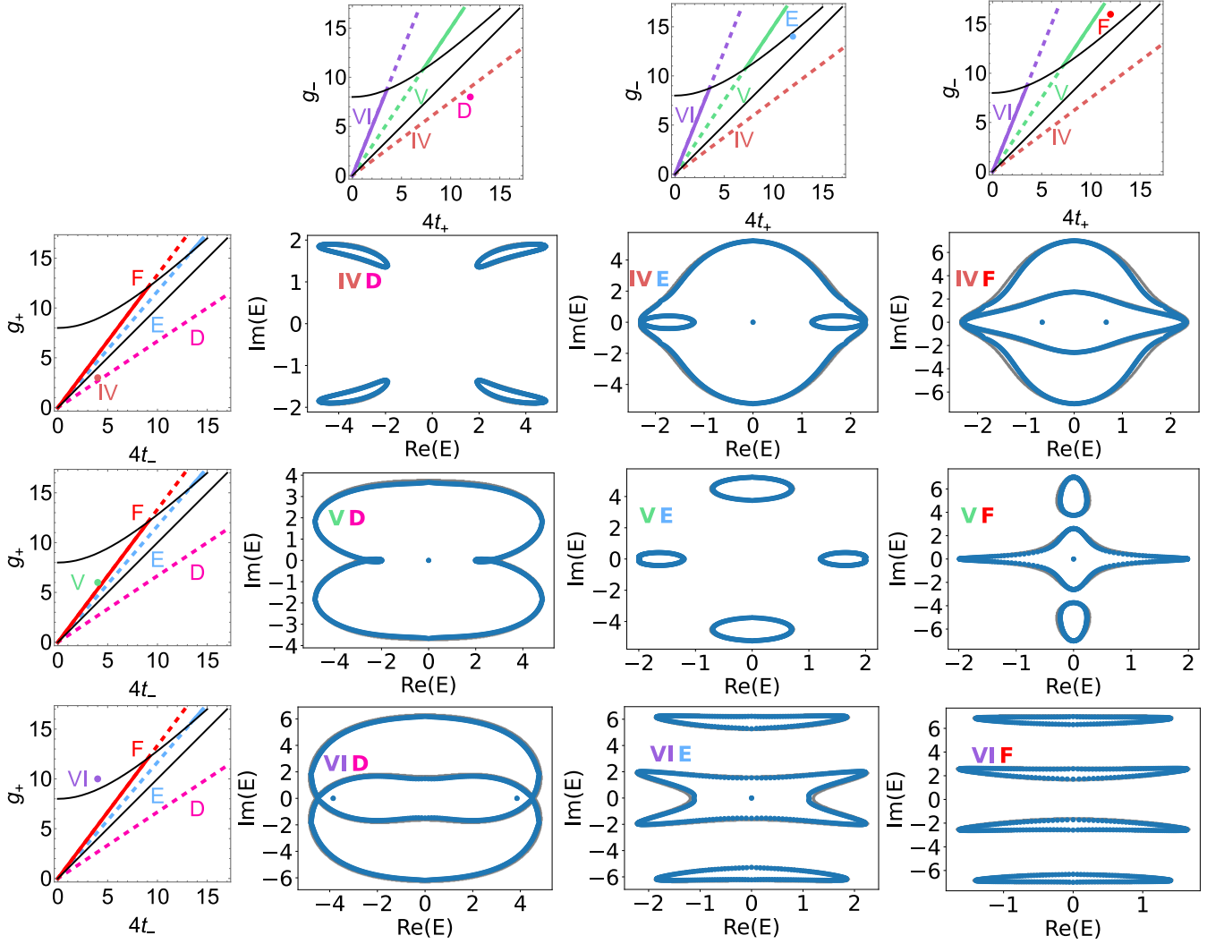
FIG. 6. Similar plots as Fig. 5, but with D_- = 0 . The representative parameter sets in the (t_-, g_+) space are labeled as IV, V and VI, and those in (t_+, g_-) space are labeled as D, E and F. See Table III for the adopted values of the full parameter sets.
