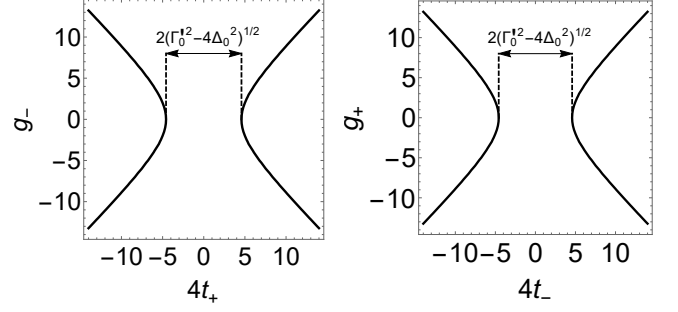
FIG. 10. Gap closing curves in the t_+-g_- (left) and t_--g_+ (right) space in the staggered limit. The adopted parameter values are given by \Gamma'_0 = 5 and \Delta_0 = 1 .
