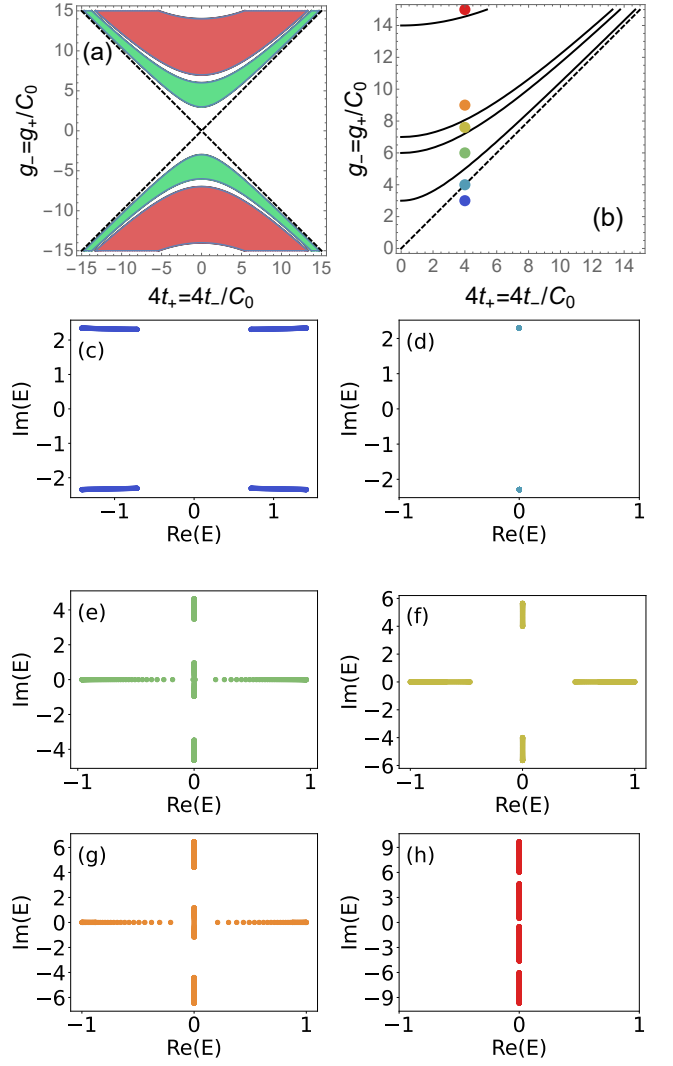
FIG. 3. (a,b) Phase diagrams and (c-h) energy spectra for Case (iib), where Eqs. (10)–(11) hold with C_0 = 0.5 ; in this case, g_\pm and t_\pm are mutually dependent. (a) Phase diagram with gapless superconducting phase in the shaded regions. (b) The first quadrant of Panel (a), with dots indicating parameter sets of t_+ = 1 and g_- = 3, 4, 6, 7.6, 9 , and 15 at \Gamma_0 = 5.0 and \Delta_0 = 1.0 , which are marked by the corresponding colors to the energy spectra in Panels (c–h). Here, the PBC spectra coincide with the OBC ones.
