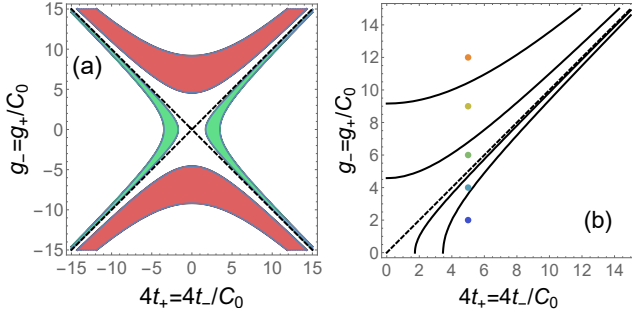
FIG. 9. Phase diagrams and energy spectra for Case (iib') with \Gamma_+ = 3 , \Gamma_- = 2 , \Delta_0 = 1 , and C_0 = 0.5 . (a) Phase diagram. The shaded regions show the gapless superconducting phases given by Eq. (27a). (b) A magnified view of the first quadrant of Panel (a), with the dot colors corresponding to the spectra in Fig. 13 (see below).
