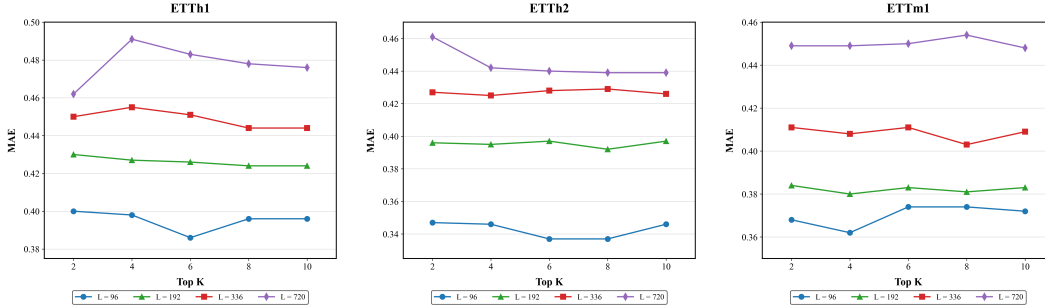
Figure 4: Influence of the selection of Top-K in different prediction length (L). We choose ETTh1, ETTh2 and ETTm1 for visualization.
