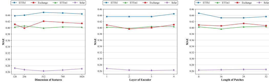
Figure 5: Influence of the hidden dimension of features, number of encoder layers and patch length. We select ETTh1, ETTm1, Exchange and Solar-Energy for visualization.
