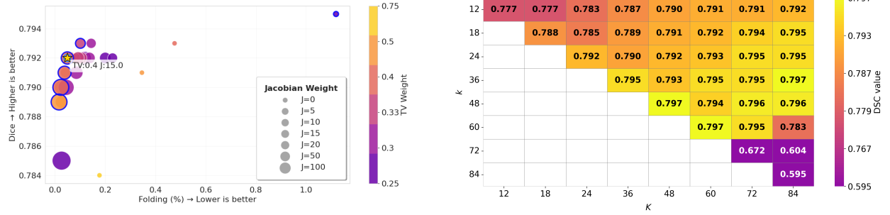
Figure 4: Left: Ablation study of loss weights for RandKAN-IDIR model on the OASIS-1 dataset. Configurations on the Pareto frontier are highlighted in blue. Right: Ablation study of k and K parameters for RandKAN-IDIR model on the OASIS-1 dataset.
