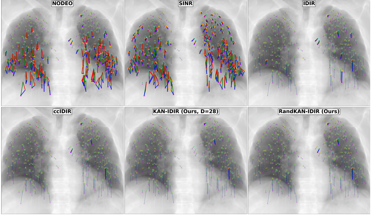
Figure 3: Landmark alignment in DIR-Lab Dataset (Case 7) for fixed, moving, and moved images. Displacements are shown as: blue (method result, moved-to-fixed), green (ground truth, moving-to-fixed), and red (error, moved-to-fixed). Landmarks with errors exceeding 3 mm are highlighted in bold, while others are displayed as transparent. Results reflect each method’s optimal seed (minimum mean TRE across 10 runs). Proposed KAN-IDIR and RandKAN-IDIR achieve the fewest outliers. The best seed-dependent variability of the proposed methods is demonstrated in Figure 5 in Appendix using worst-case (maximum mean TRE) results.
