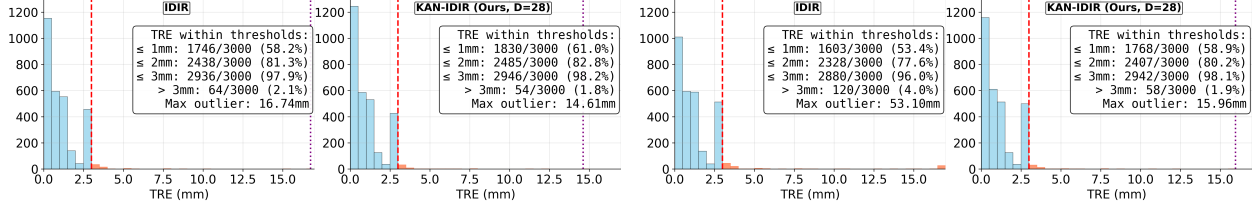
Figure 1: Target registration error (TRE) distributions for IDIR and proposed KAN-IDIR across all DIR-Lab cases, comparing outlier characteristics between optimal ( lowest mean error ; first two histograms) and suboptimal ( highest mean error ; last two histograms) seed initializations from a total of 10 seeds. The dashed red line indicates the 3 mm acceptability threshold, while the dotted purple line marks the maximum outlier value per method. Our proposed KAN-IDIR demonstrates: (1) fewer outliers overall in optimal seed conditions – 54 vs. 64 for IDIR; and (2) consistent performance across seed selections – > 3mm outlier count difference for best/worst seed is 4 for KAN-IDIR vs. 56 for IDIR.
