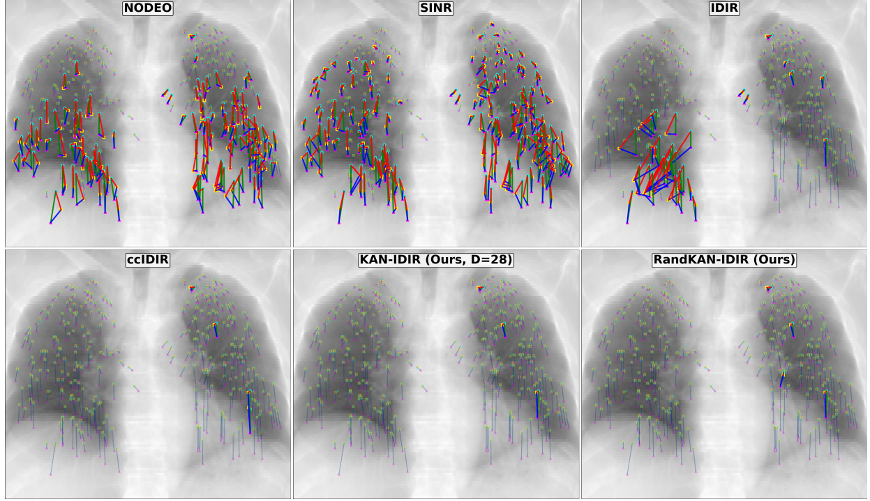
Figure 5: Landmark alignment in DIR-Lab Dataset (Case 7) for fixed, moving, and moved images. Displacements are shown as: blue (method result, moved-to-fixed), green (ground truth, moving-to-fixed), and red (error, moved-to-fixed). Landmarks with errors exceeding 3 mm are highlighted in bold, while others are displayed as transparent. Results reflect each method’s suboptimal seed (maximum mean TRE across 10 runs). Proposed KAN-IDIR and RandKAN-IDIR still achieve the fewest outliers, while the other methods demonstrate significant increase.
