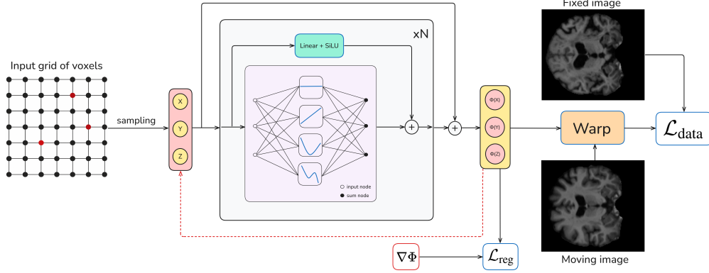
Figure 2: The overall pipeline of the proposed method for deformable image registration. Voxels are sampled from the input volume to serve as input to the KAN-IDIR or RandKAN-IDIR models. The network outputs a deformation field, which is used to warp the moving image, enabling calculation of the data similarity loss. For regularization, the gradient of the deformation field is computed using automatic differentiation.
