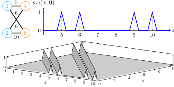
Figure 1: Spike function s_{r,l} for a colored graph (top left). Node labels: \omega_{r,1} = 1, \omega_{r,2} = 2, \omega_{l,1} = 4, \omega_{l,2} = 8 . Edge labels: \omega_{r,1,l,1} = 5, \omega_{r,2,l,1} = 6, \omega_{r,1,l,2} = 9, \omega_{r,2,l,2} = 10 .
