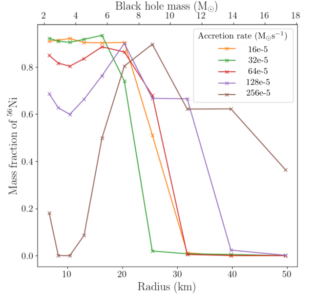
Figure 8. ^{56}\text{Ni} mass fraction as a function of the position in the accretion disk. The innermost radius depends upon the mass of the black hole. The innermost stable circular orbit for a maximally rotating black hole dictates the innermost radius of the disk. The upper x-axis shows the position of the innermost disk radius for a set of black hole masses at maximal spin. The ^{56}\text{Ni} in the disk drops precipitously when the black hole exceeds 5 M_{\odot} for all accretion rates expected for helium mergers. Lower-mass black holes will produce some ^{56}\text{Ni} , but we expect the total yield to be low (Abrahams et al. 2023).
