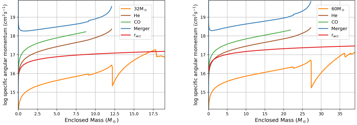
Figure 5. Specific angular momentum versus mass coordinate for a single star with moderate dynamo models locking different burning layers, tidally-locked Helium and CO star collapsars (Fryer et al. 2019, 2025), and our helium star merger model. The two plots show the results for the cores produced by two different 1/10th solar, stellar models (32 and 60 M_{\odot} zero-age main sequence stars) at CO depletion. A powerful jet requires an accretion disk at \sim 100 km, i.e. viable GRB models must exceed the red line above.
