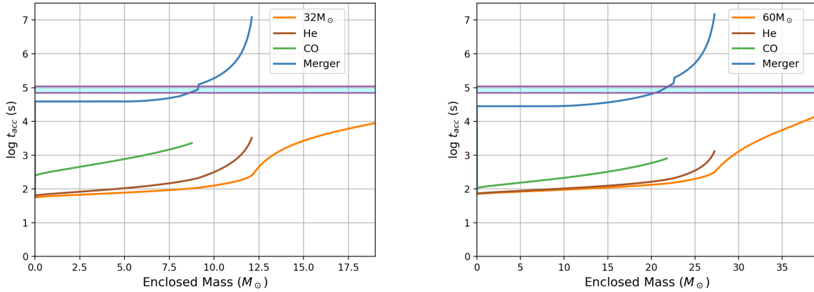
Figure 6. Accretion timescales versus mass coordinate for the models in Fig. 5. The timescales for single stars are dominated by the free-fall time, but the accretion timescale for helium-mergers is entirely set by the disk accretion timescale. Our inferred central engine duration is shown as a horizontal line, where only the helium star merger is remotely viable.
