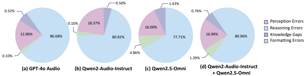
Figure 6: Distribution of error types in the responses of four models. Reasoning errors remain the primary type of errors in the responses of LALMs, followed by perception errors.
