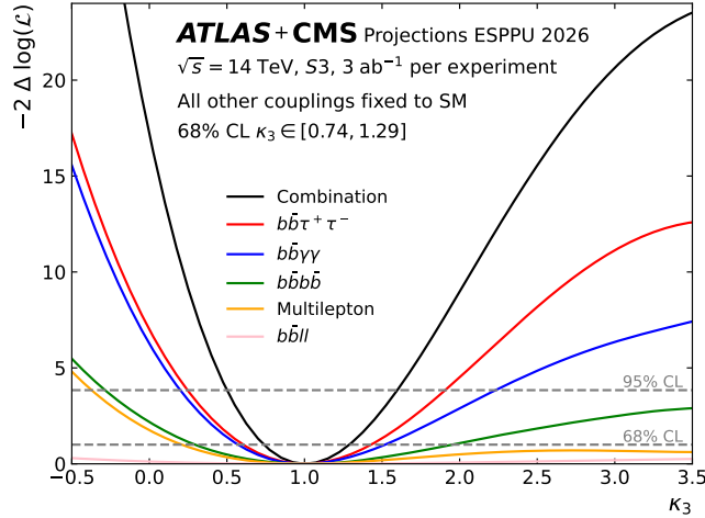
Fig. 10. Contributions to the \chi^2 distribution of various analysis channels and their combination as a function of \kappa_3 for the S3 scenario 3 ab -1 . From [17].
