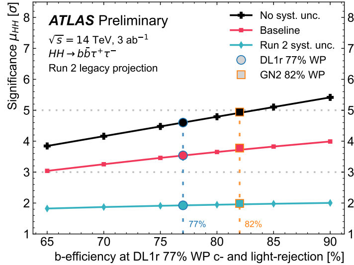
Fig. 11. Dependence of the HH detection significance as a function of the b -tagging efficiency for the scenarios with Run-2 systematic uncertainties, the baseline (S3) and without systematic uncertainties. From [20].
