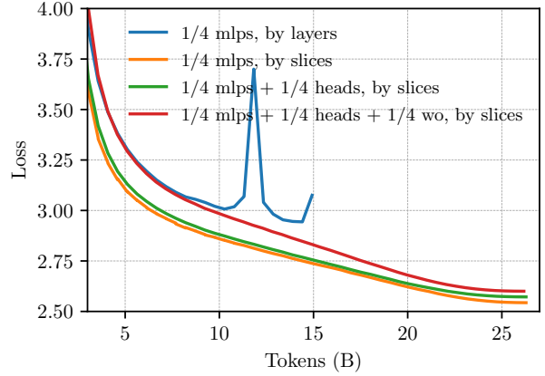
Figure 5 Test loss as a function of training tokens for different variants of trainable parameter assignment. “By layers” corresponds to training only a subset of layers on each node – slicing model horizontally, whereas “by slices” refers to slicing parameters vertically as described in § 2.2.1.
