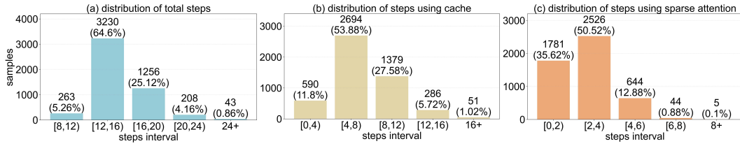
Figure 9: Visualization of distribution patterns in dynamic acceleration strategies. In (a), we visualize the distribution of total steps for sample generation. In (b) and (c), we demonstrate the distribution of steps using cache and sparse attention. For instance, 3,230 samples are generated using 12–16 steps, 2,694 samples utilize cache reuse with 4–8 steps, and 2,526 samples employ sparse attention with 2–4 steps during the generation process. This experiment is based on our model, which achieves a 2.91 \times speedup over FLUX Labs (2024), as illustrated in Figure 3.
