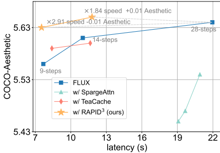
Figure 3: Latency vs. quality trade-off. Figure 4: Visual comparison. The acceleration ratio relative to the original FLUX 28-steps is reported.
