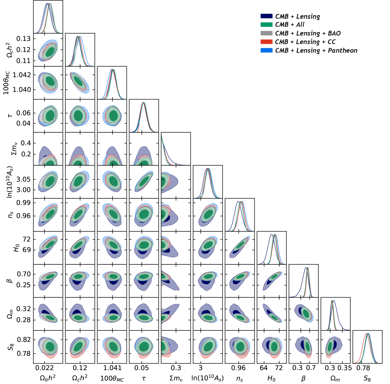
Figure 2: Comparison results of the S_8 , \Omega_b h^2 , \Omega_c h^2 , \beta , \tau , n_s , \ln(10^{10} A_s) , 100\theta_{MC} , H_0(km/s/Mpc) for different combination dataset for Coupled quintom to neutrinos.
